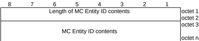
Figure J.1.5-1: MC Entity ID information element
