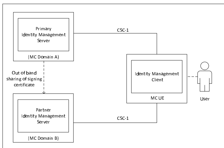
Figure 5.1.4.2-1: Functional Model for Inter-Domain Identity Management
