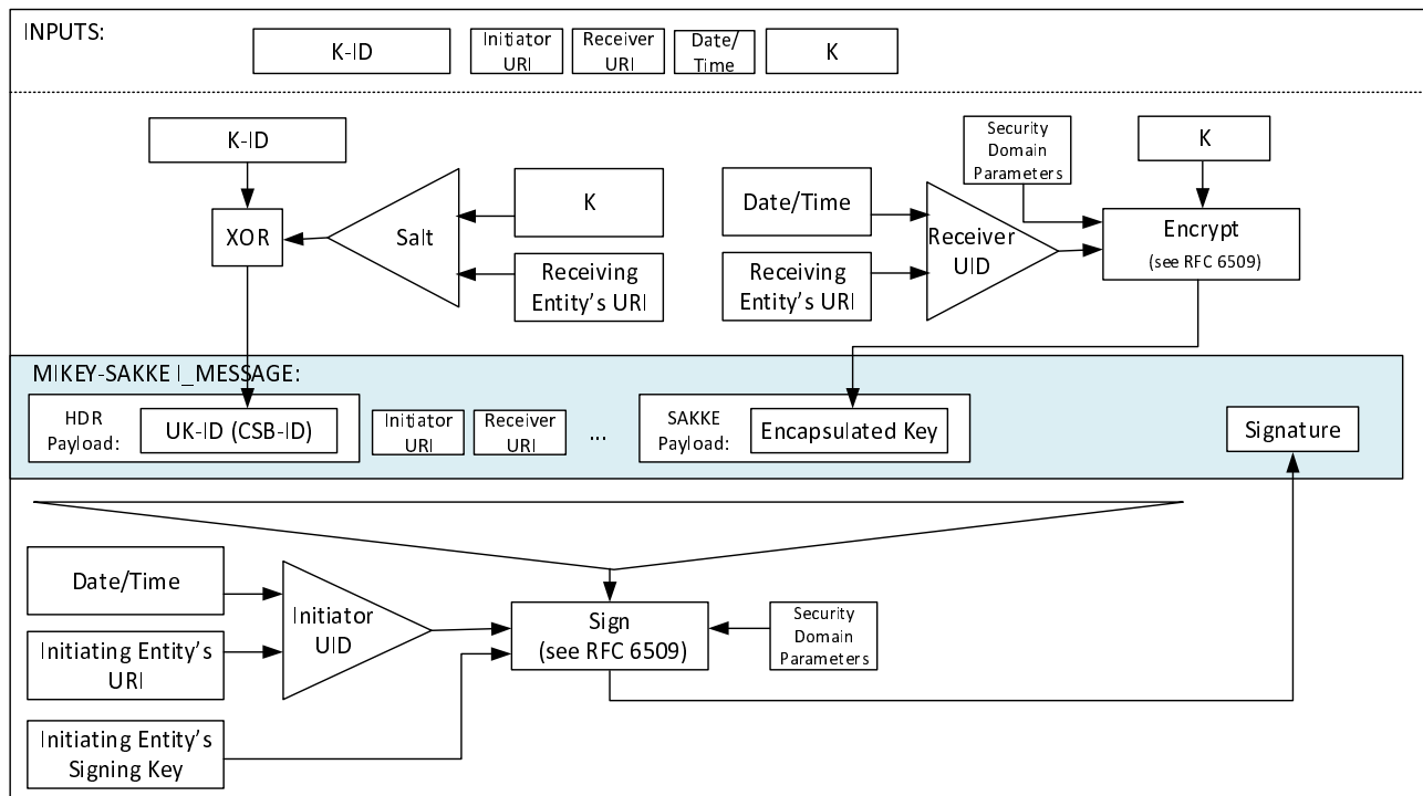
Figure 5.2.3-2: Common key distribution mechanism with end-point diversity
