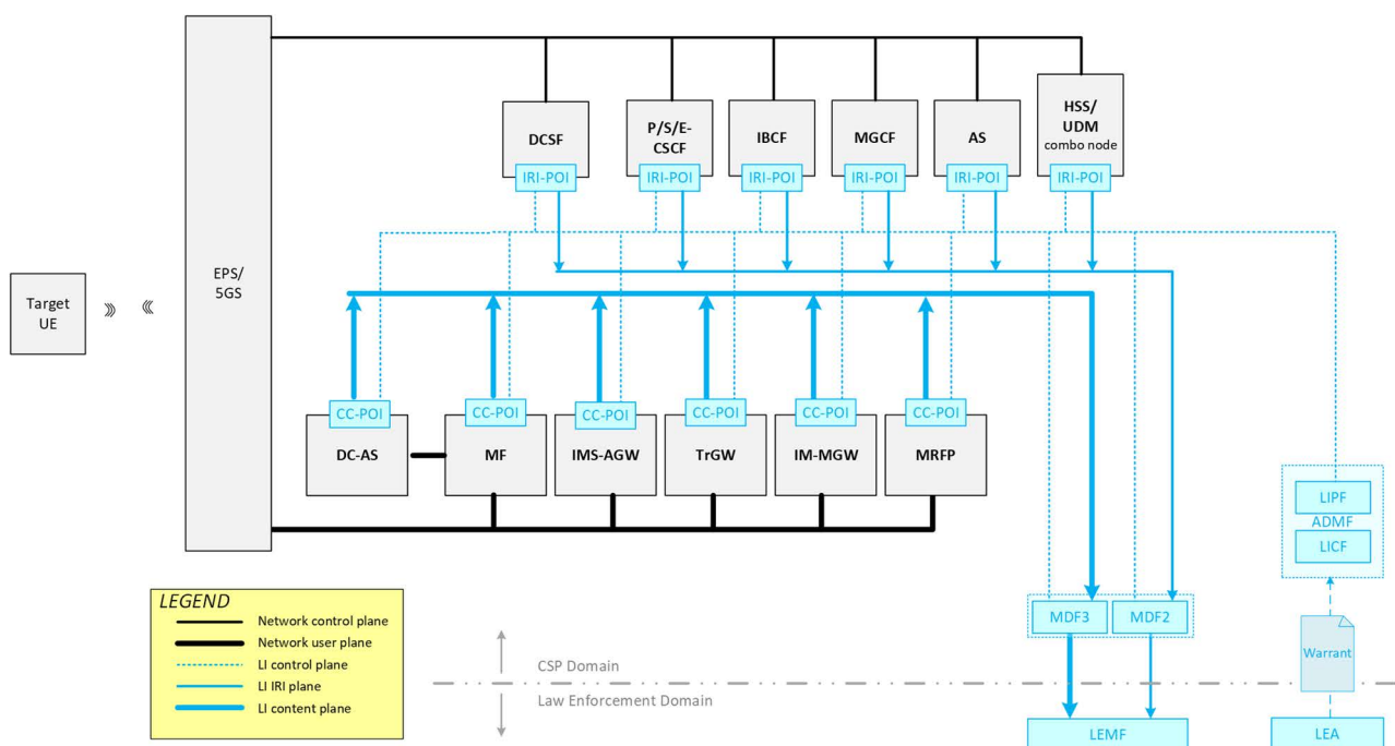
Figure 7.4-1: EPS/5GS-Anchored IMS High Level LI Architecture
