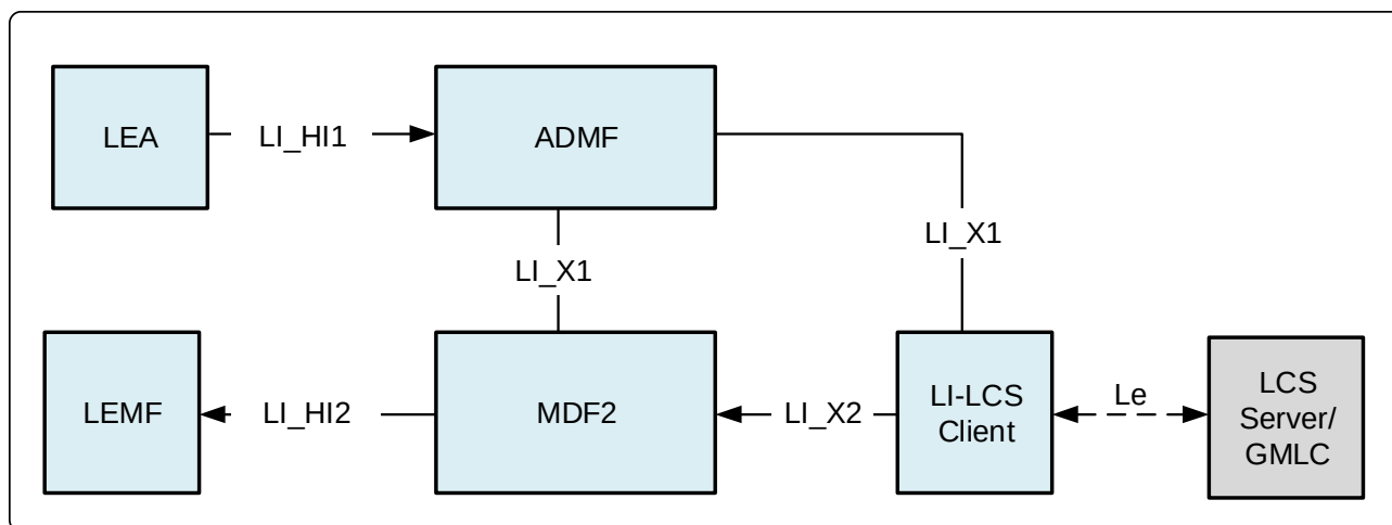
Figure 7.3-1: LALS model for target positioning
