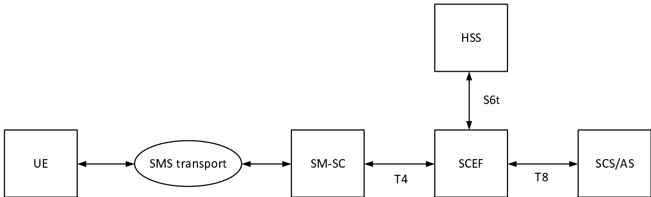
Figure 7.11-2: EPS architecture for device triggering
