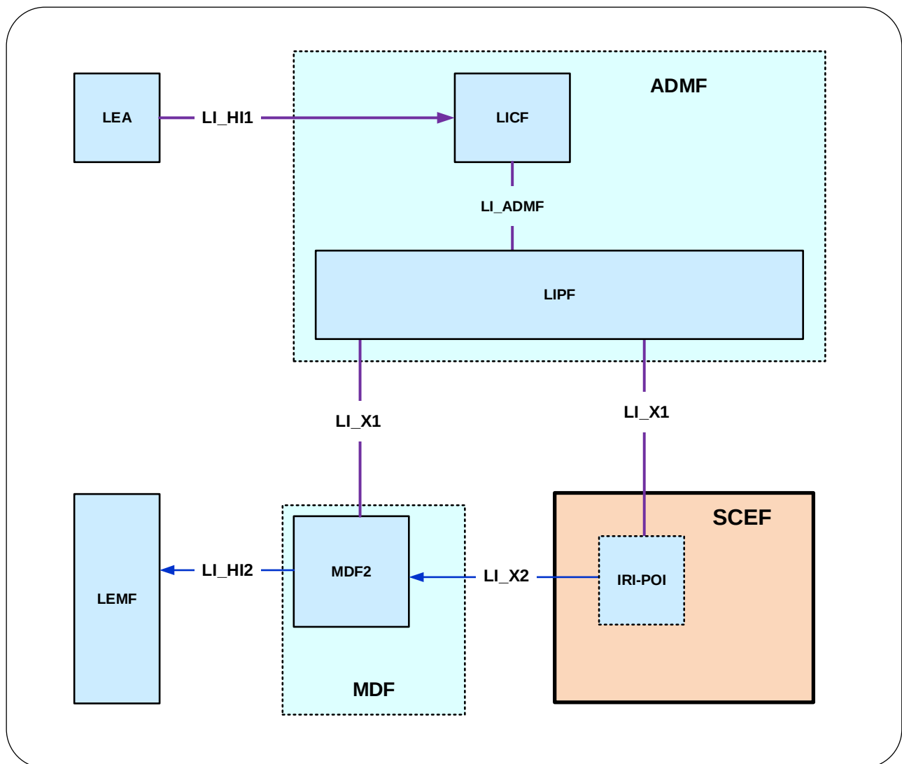
Figure 7.11.3.2-1: LI architecture for device triggering using SCEF
