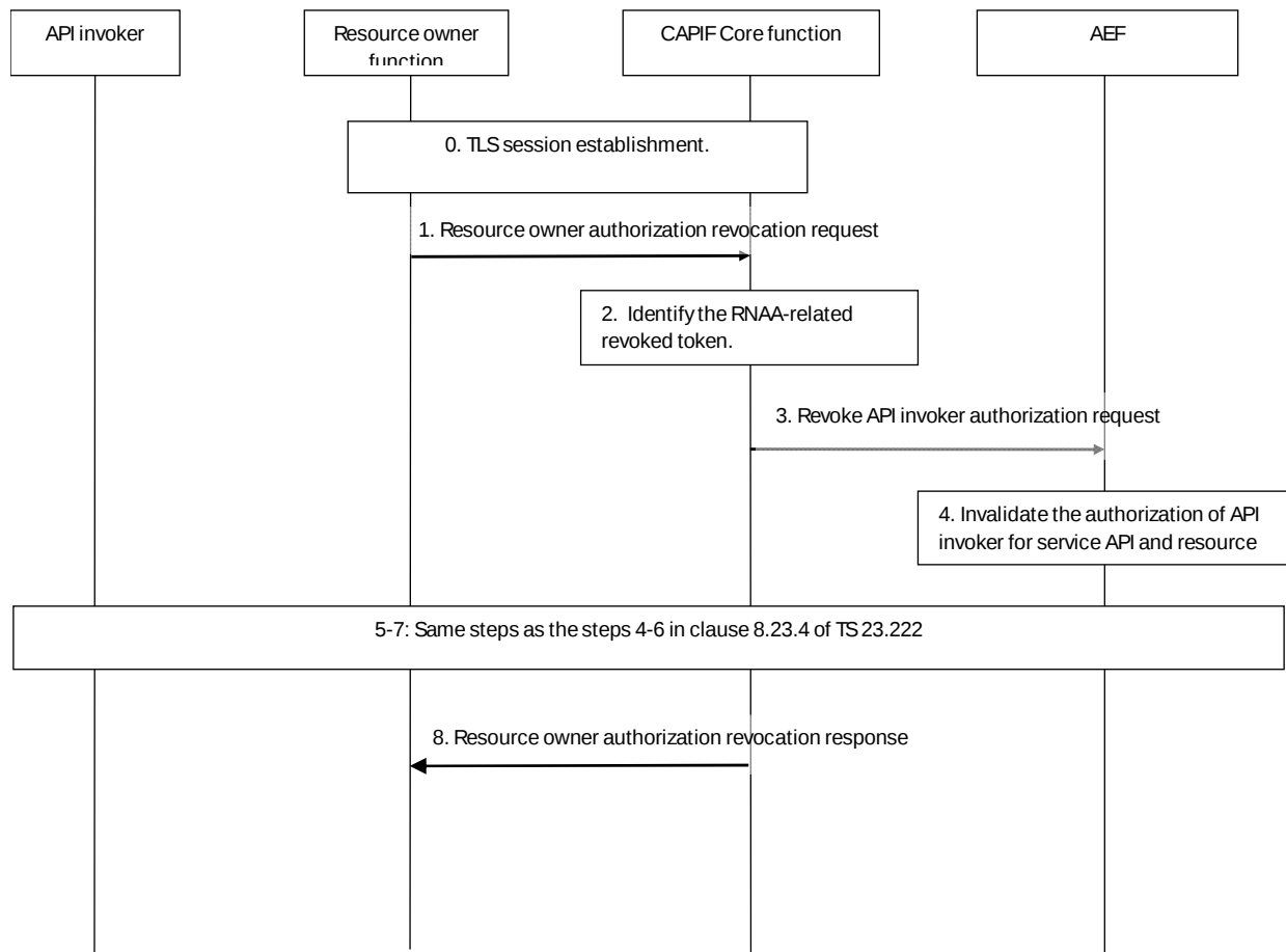
Figure 6.5.3.4-1: Procedure for revoking resource owner authorization
