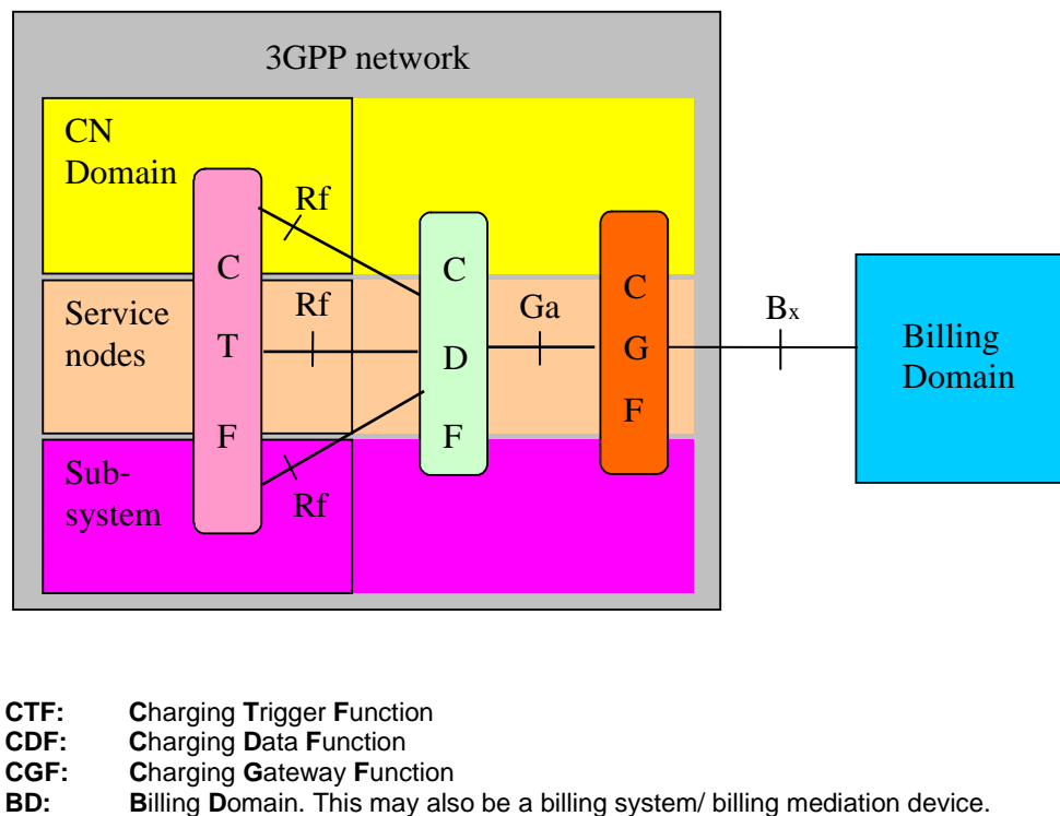
Figure 4.1: Logical ubiquitous offline charging architecture
