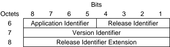
Figure 6.4.1: The format of the Data Record Format Version field
