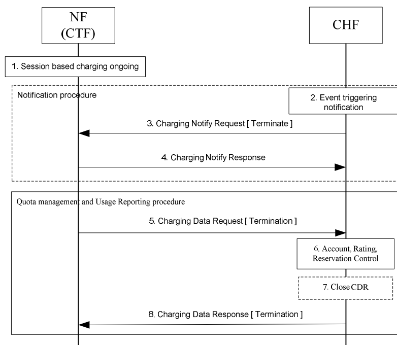
Figure 5.3.2.4.2: Session based charging – Notification with termination
