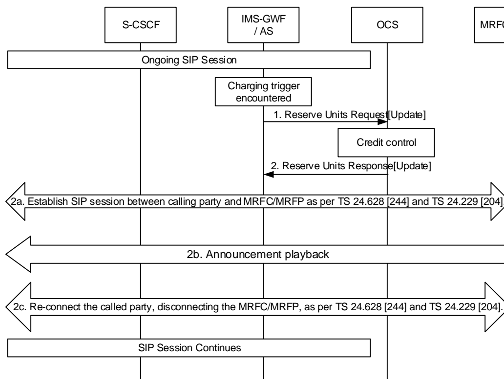
Figure 5.2.2.3: Message sequence chart for mid-quota announcement during IMS session
