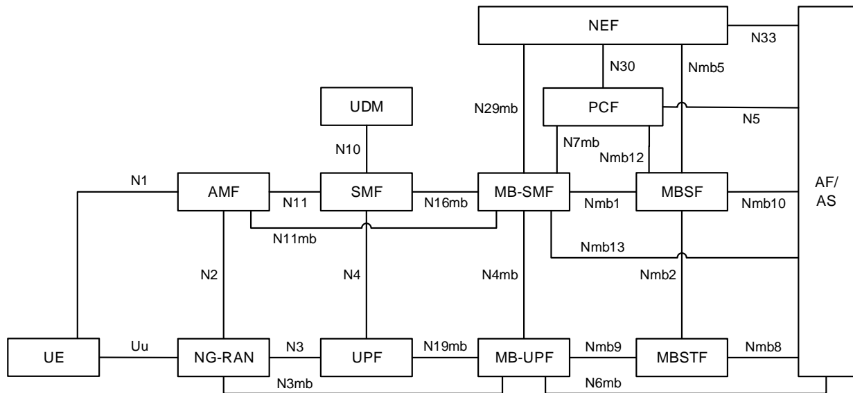
Figure 4.1-1: Non-roaming architecture for 5G Multicast and Broadcast Service in reference point representation
