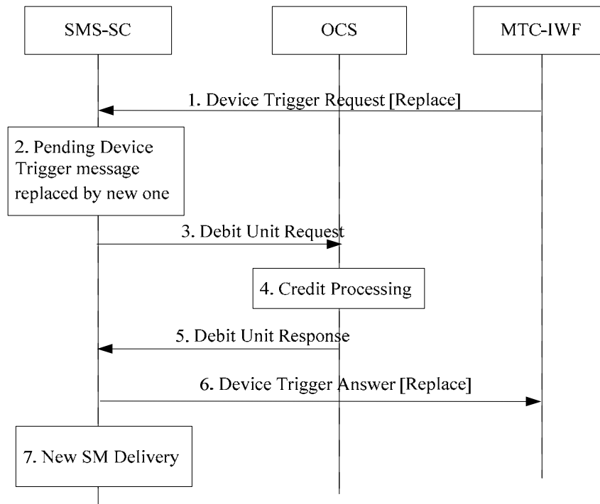
Figure 5.3.2.11.4.1: Online charging - SMS submission to SMS-SC for replace Device Triggering
