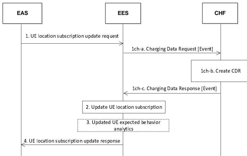
Figure 5.2.4.2.6.6-1: Charging for UE location subscription - IEC
