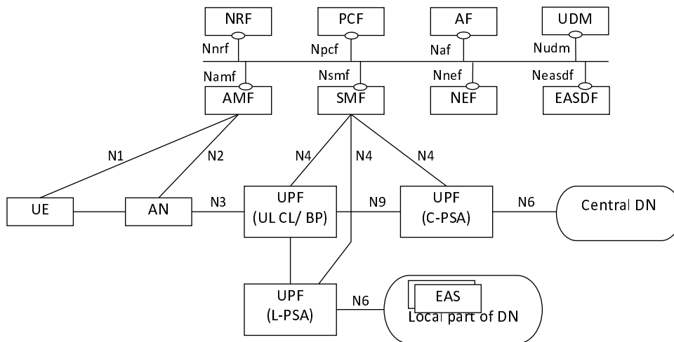
Figure 4.1.1.1-1: 5GS providing access to EAS with UL CL/BP for non-roaming scenario
