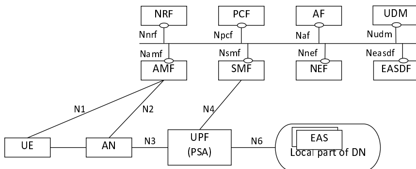
Figure 4.1.1.1-2: 5GS providing access to EAS without UL CL/BP for non-roaming scenario
