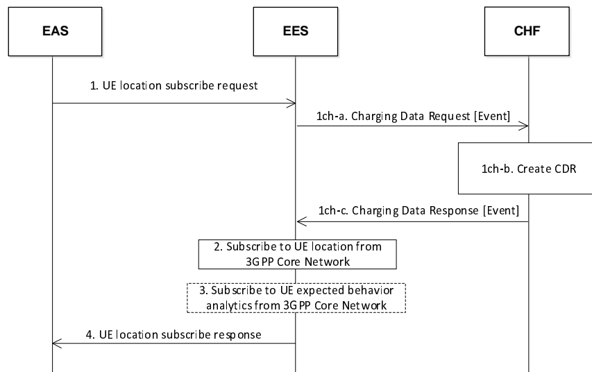
Figure 5.2.4.2.6.4-1: Charging for UE location subscription - IEC
