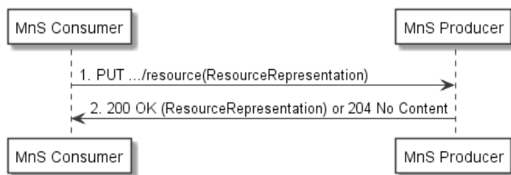
Figure 5.3-1: Flow for updating a resource
