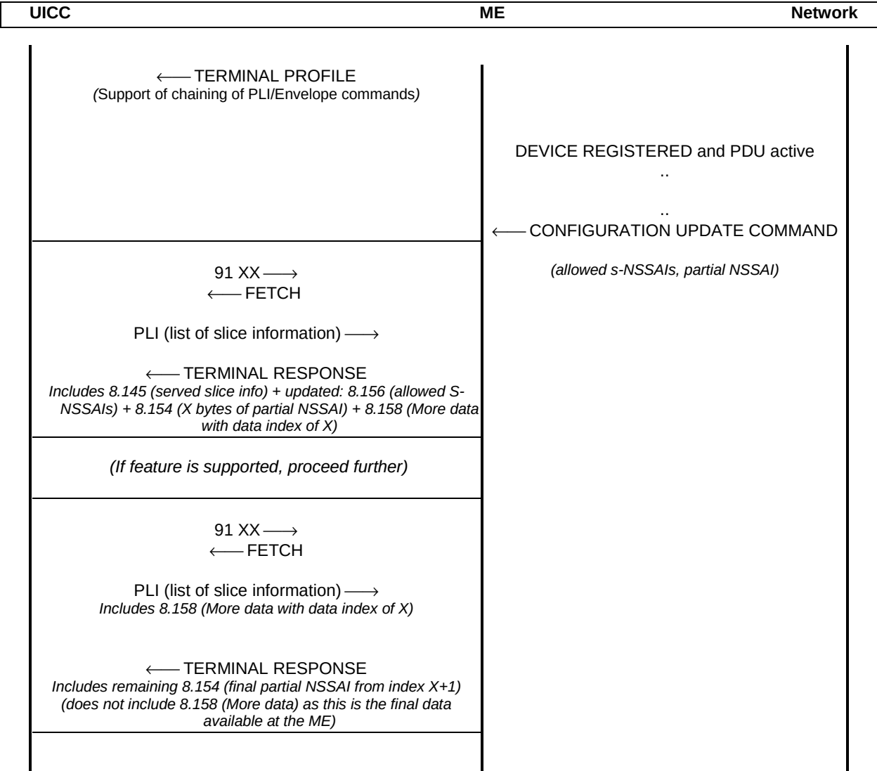
Figure V.2.1 slice status change procedure (providing the full list of partial NSSAI information)
