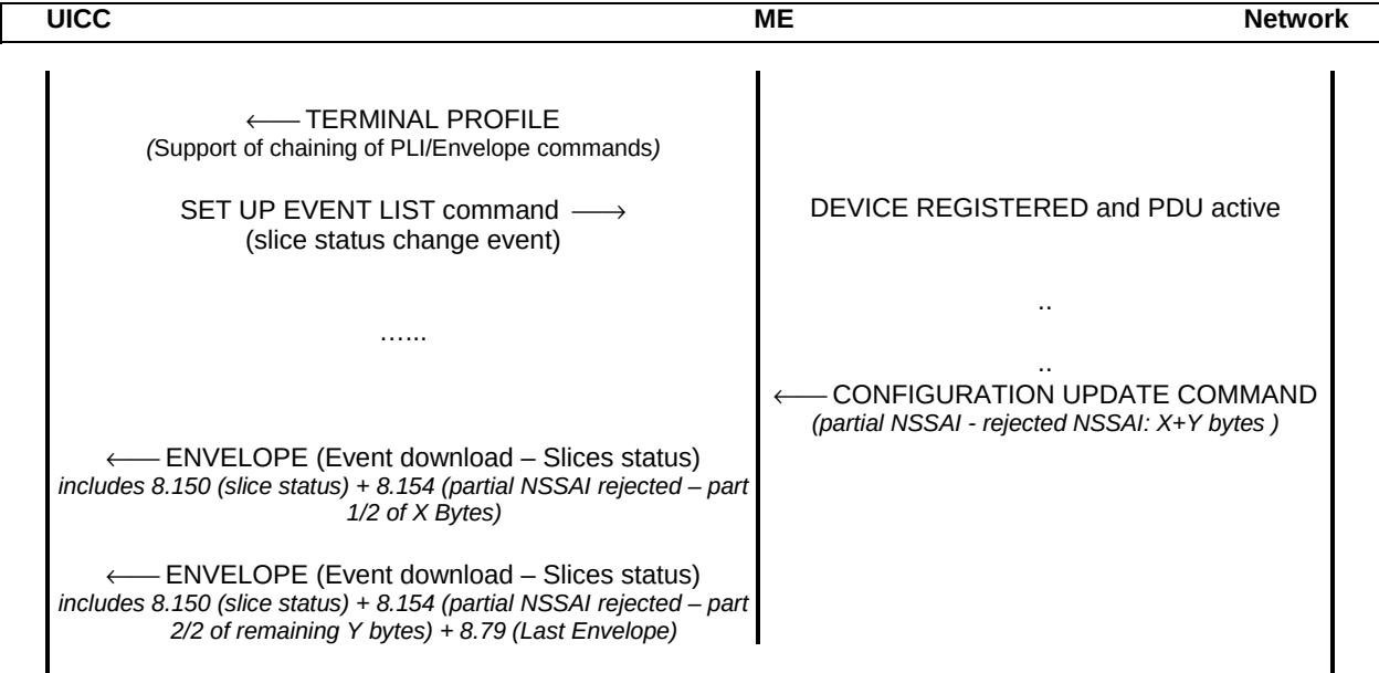
Figure U.2.1 slice status change procedure (providing the full list of partial NSSAI information)
