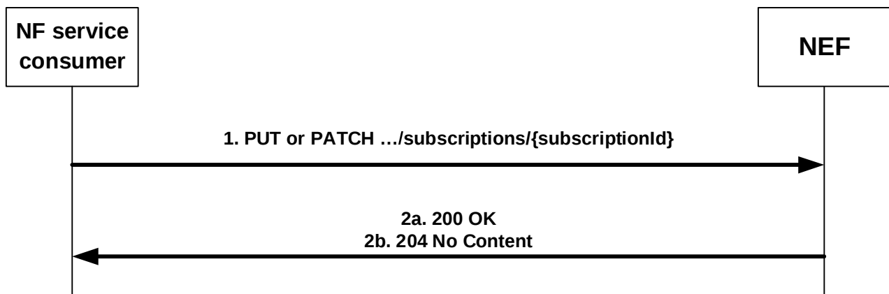
Figure 4.5.2.2.3-1: Modification of an existing subscription
