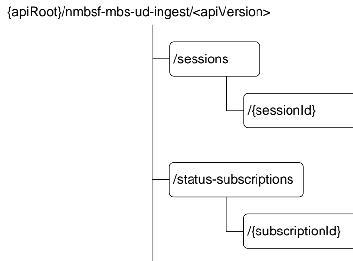
Figure 6.2.3.1-1: Resource URI structure of the Nmbfs_MBSUserDataIngestSession API
