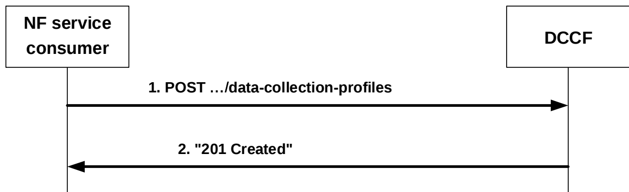
Figure 4.3.2.2.2-1: NF service consumer registers data collection profile
