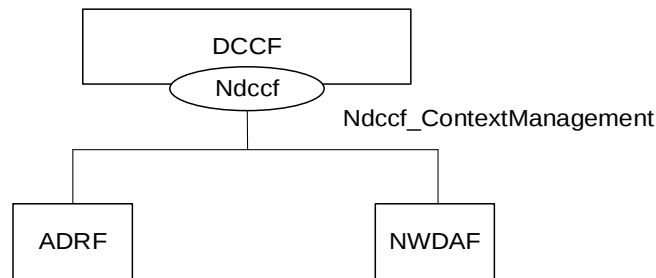
Figure 4.3.1.2-1: Ndccf_ContextManagement service architecture, SBI representation
