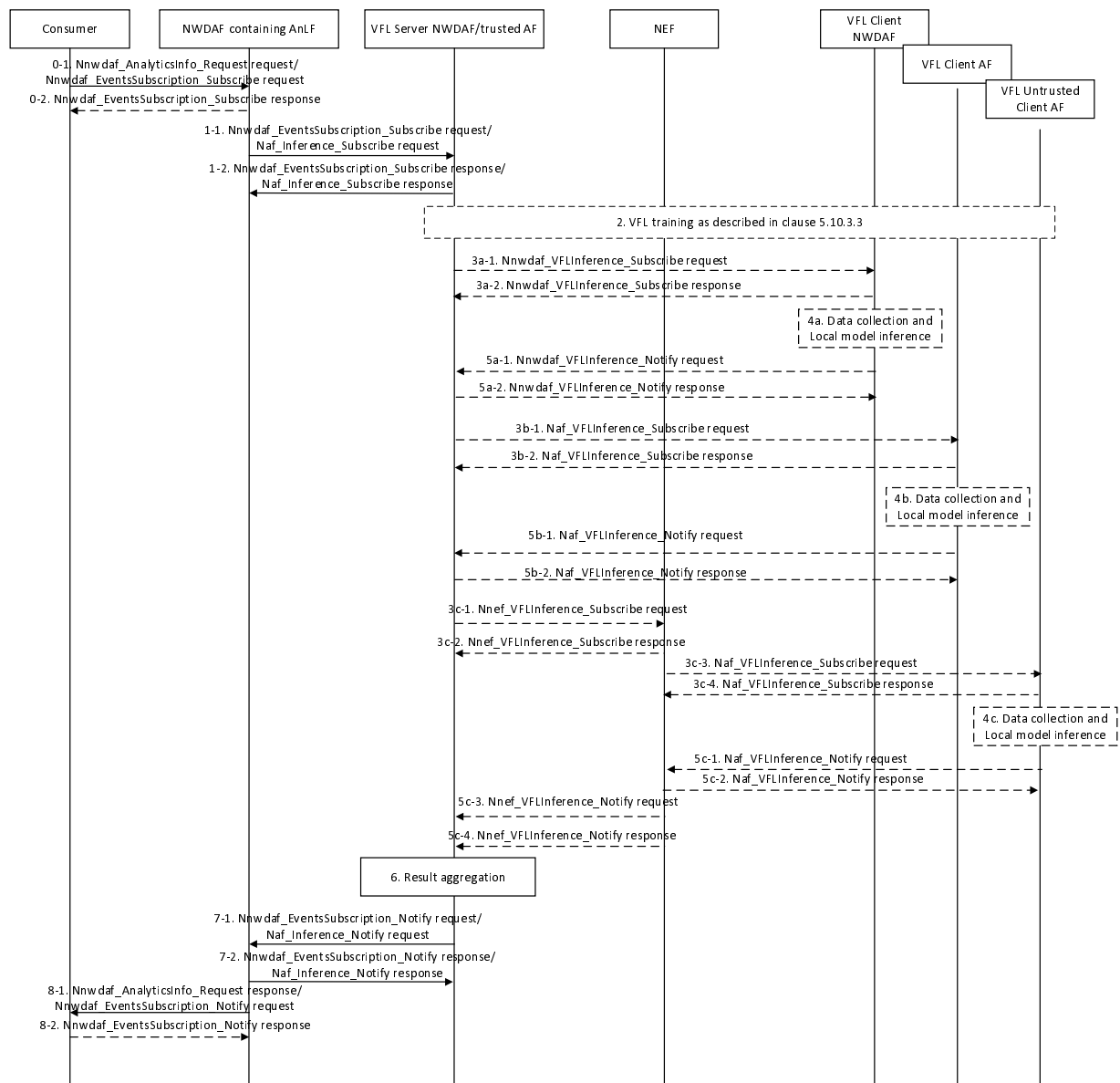
Figure 5.10.3.4.2-1: General procedure for Vertical Federated Learning when NWDAF is acting as VFL server
