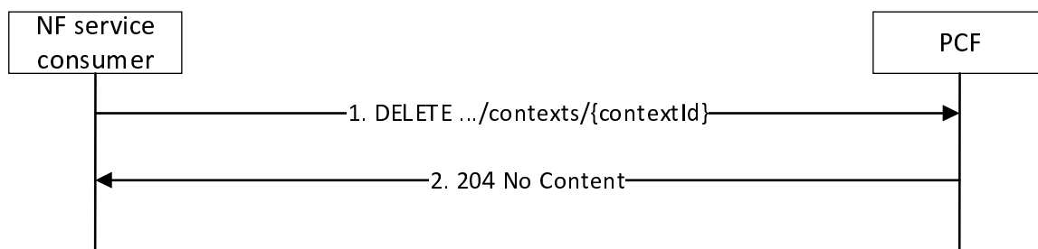
Figure 5.3.2.4.2-1: MBS Application Session Context deletion procedure
