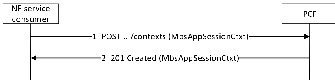
Figure 5.3.2.2.2-1: MBS Application Session Context establishment procedure
