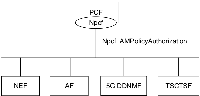
Figure 4.1.2-1: Npcf_AMPolicyAuthorization service architecture, SBI representation
