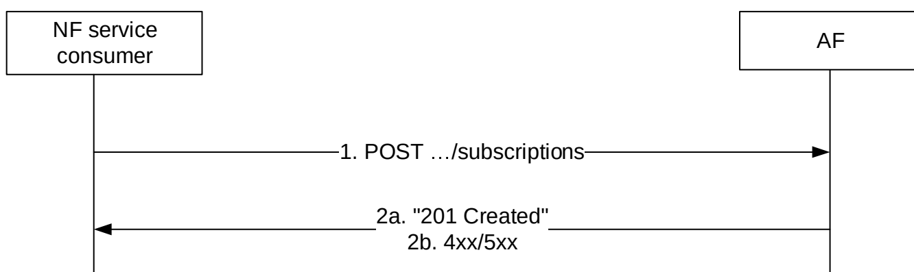
Figure 5.2.2.2.2-1: Procedure for VFL Training Subscription Creation
