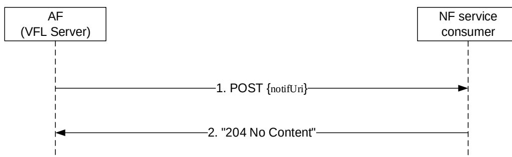
Figure 5.5.2.4.2-1: AF notifies the subscribed inference event
