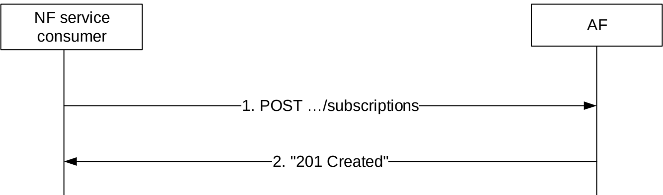
Figure 5.3.2.2.2-1: NF service consumer subscribes to VFL inference notifications
