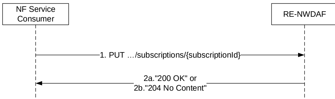
Figure 4.9.2.2.3-1: NF service consumer updates subscription to notifications
