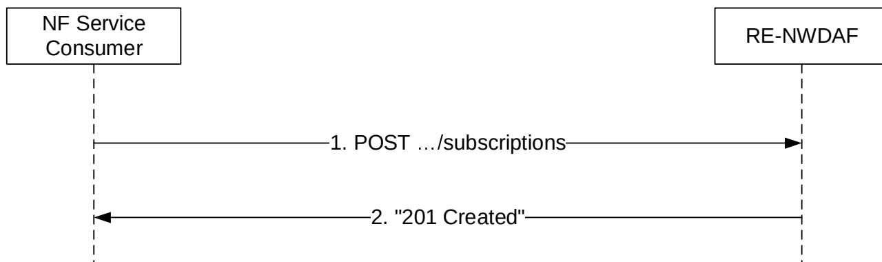
Figure 4.9.2.2.2-1: NF service consumer subscribes to notifications
