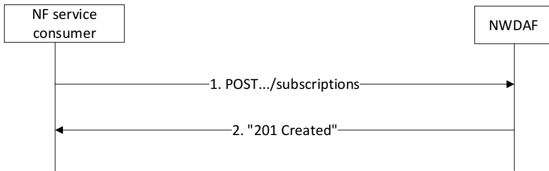
Figure 4.4.2.2-1: NF service consumer subscribes to data notifications
