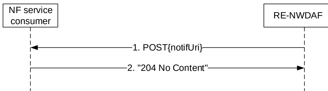
Figure 4.9.2.4.2-1: RE-NWDAF notifies the subscribed event
