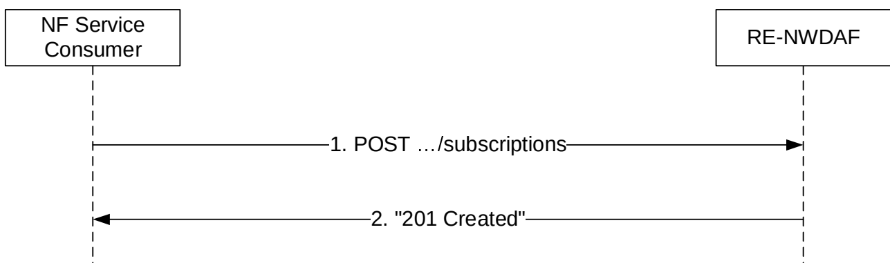
Figure 4.8.2.2.2-1: NF service consumer subscribes to notifications
