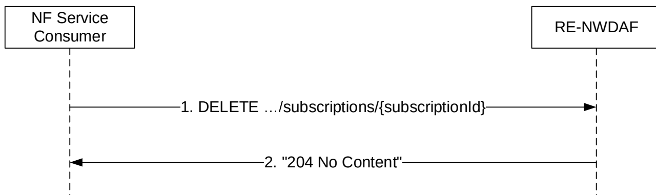
Figure 4.8.2.3.2-1: NF service consumer unsubscribes from notifications
