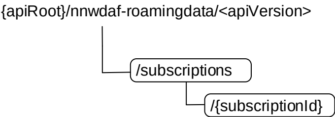
Figure 5.7.3.1-1: Resource URI structure of the Nnwdaf_RoamingData API
