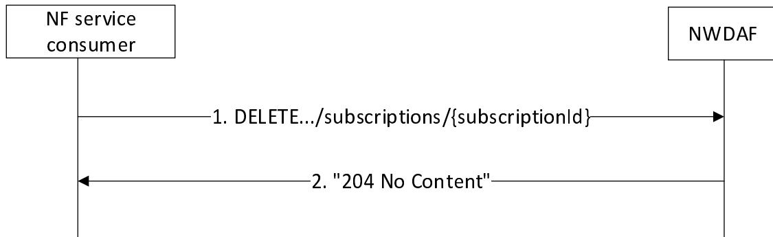
Figure 4.4.2.3.2-1: NF service consumer unsubscribes from data notifications
