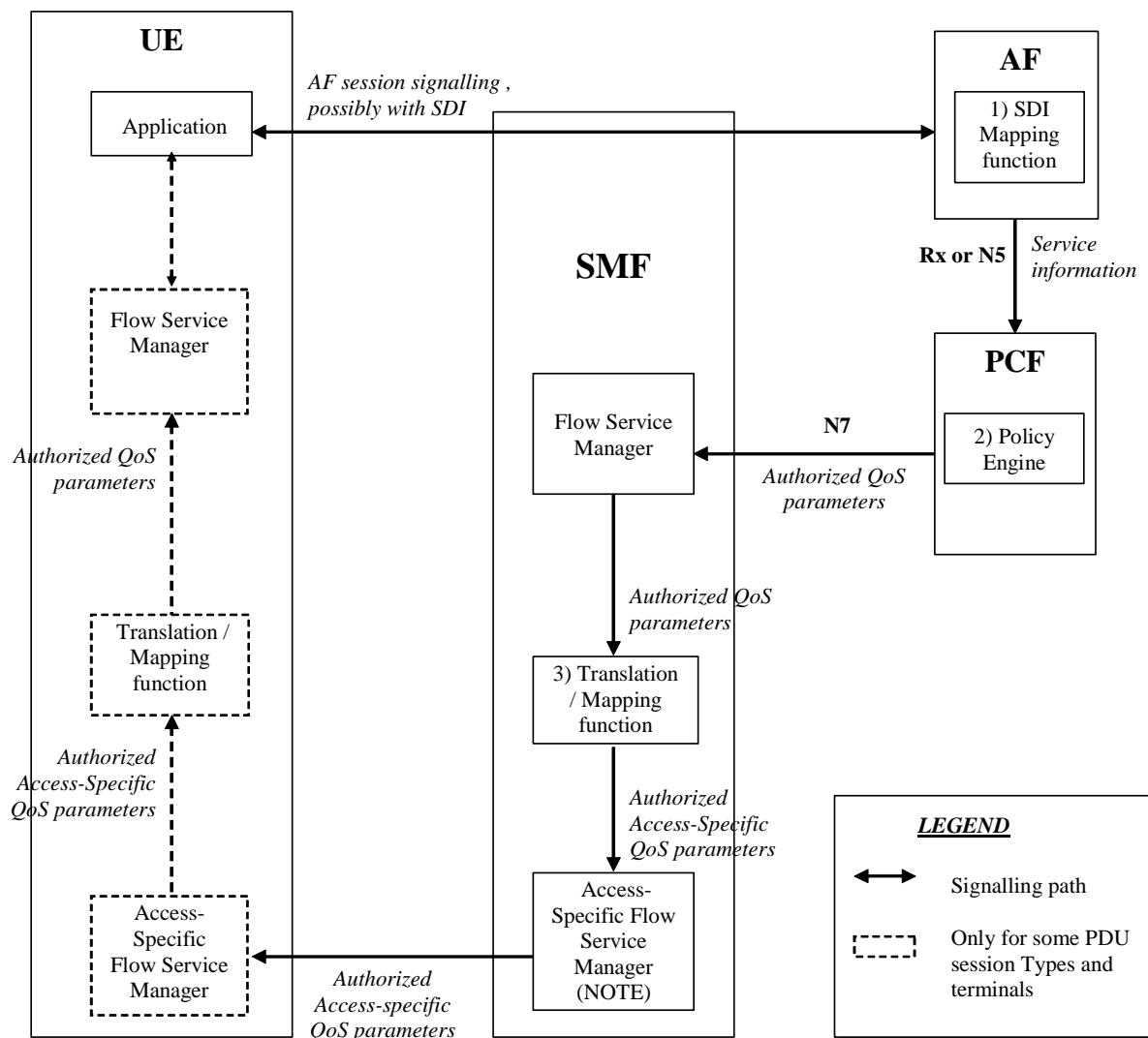
Figure 7.1-1: QoS mapping framework
