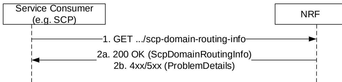
Figure 5.3.2.3-1: SCP Domain Routing Information Get
