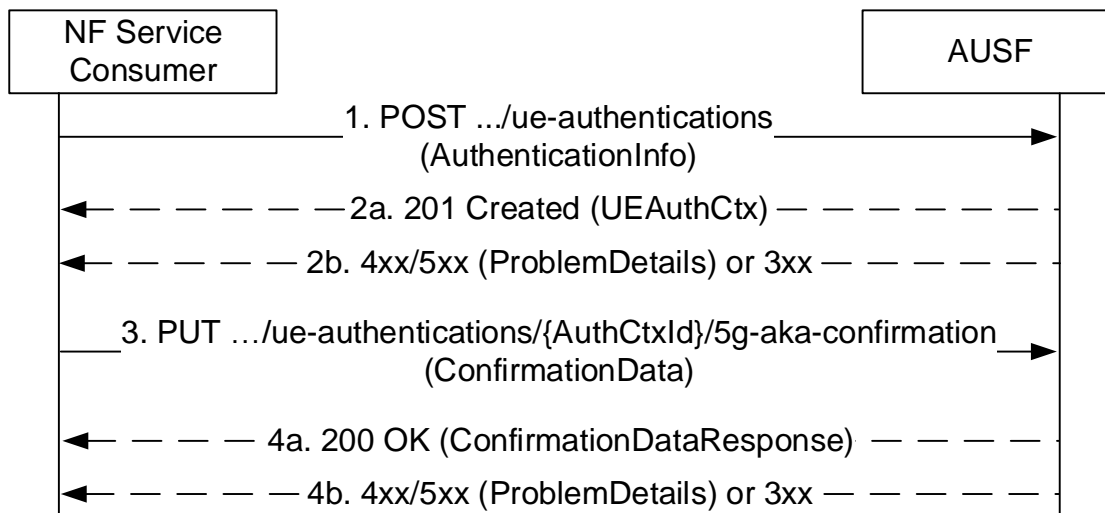
Figure 5.2.2.2-1: 5G AKA
