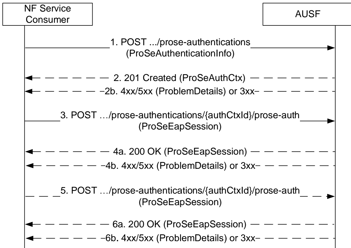
Figure 5.2.2.4.1-1: ProSe Authentication
