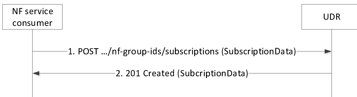
Figure 5.3.2.4.2-1: Subscribing to NF Group ID mapping changes
