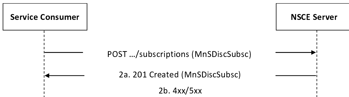
Figure 5.6.2.2.2-1: Procedure for Management Discovery Subscription Creation
