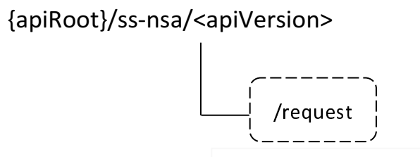
Figure 6.10.4.1-1: Custom operation URI structure of the NSCE_NetworkSliceAdaptation API
