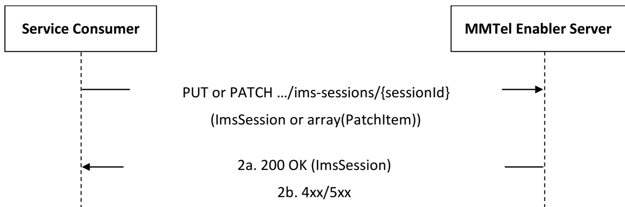
Figure 5.5.2.3.2-1: Procedure for IMS Session Update
