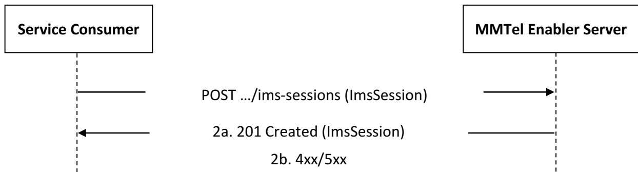
Figure 5.5.2.2-1: Procedure for IMS Session Creation
