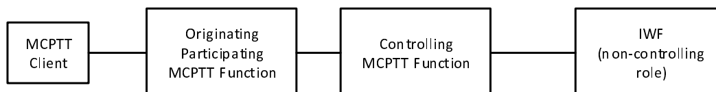
Figure 5.2-5: Relationship between the IWF and an MCPTT system with the controlling MCPTT function in the MCPTT system and a non-controlling function in the IWF
