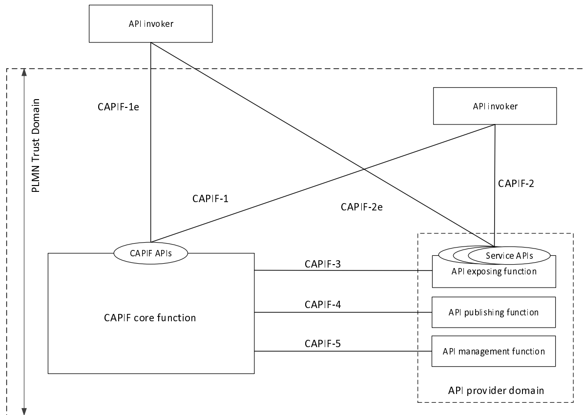
Figure 4.2-1: CAPIF Functional Model
