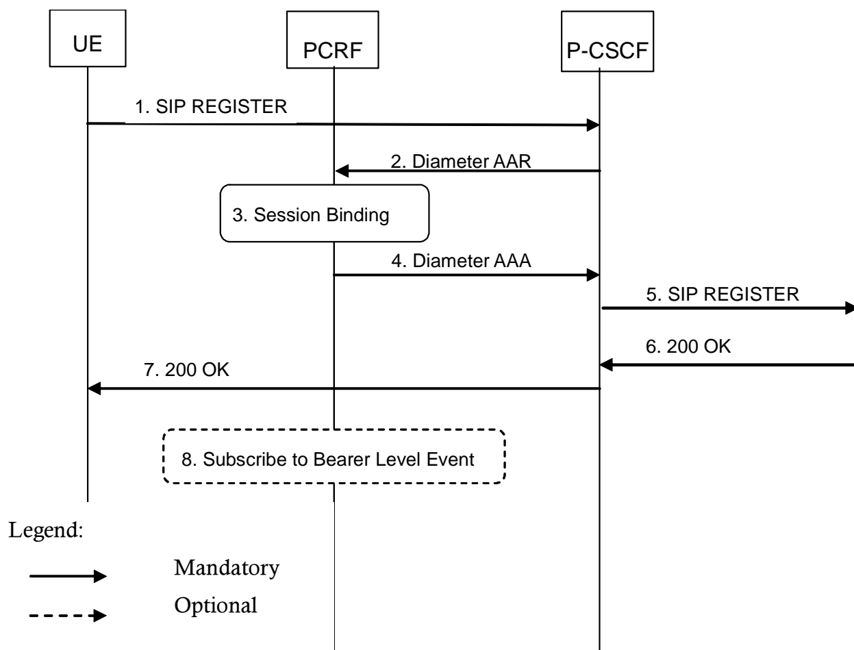
Figure B.1.2: Subscription to Notification of change of IP-CAN Type at initial IMS Registration
