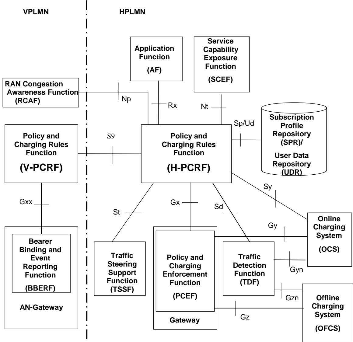
Figure 3a.2: Overall PCC architecture for roaming with home routed access scenario
