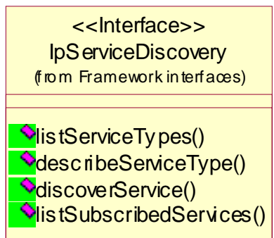
Figure: Service Discovery Package Overview
