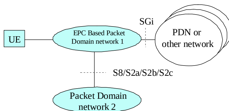
Figure 1b: EPC based Packet Domain Access Interfaces and Reference Points
