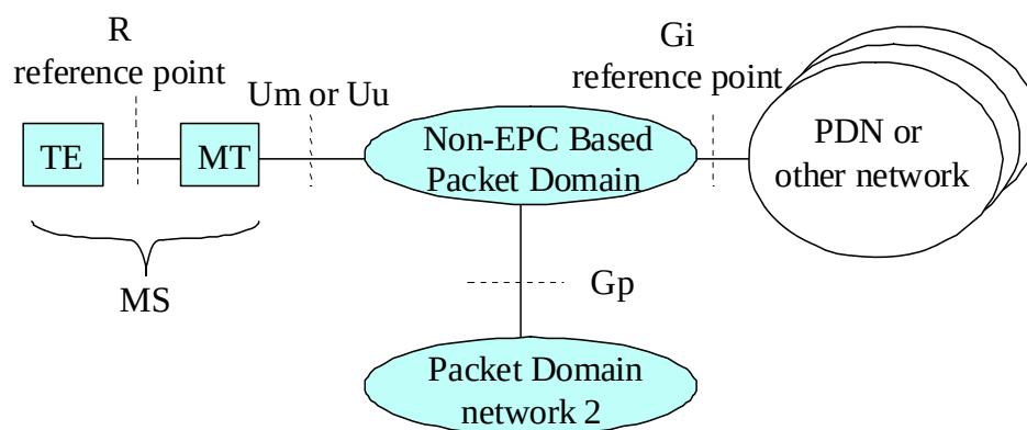
Figure 1a: Non-EPC based Packet Domain Access Interfaces and Reference Points
