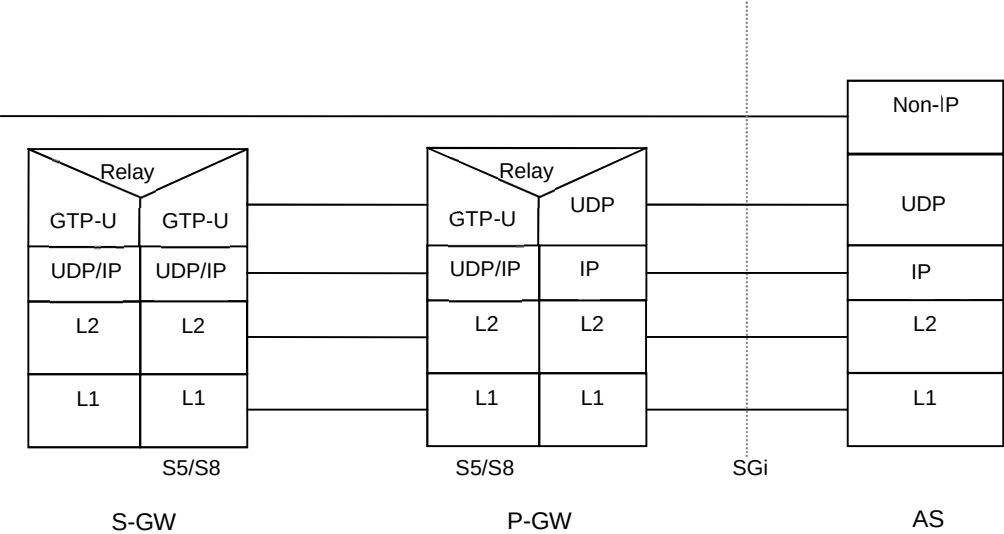
Figure 11.8: Protocol configuration for Non-IP data (user plane) using SGiPtP tunneling
