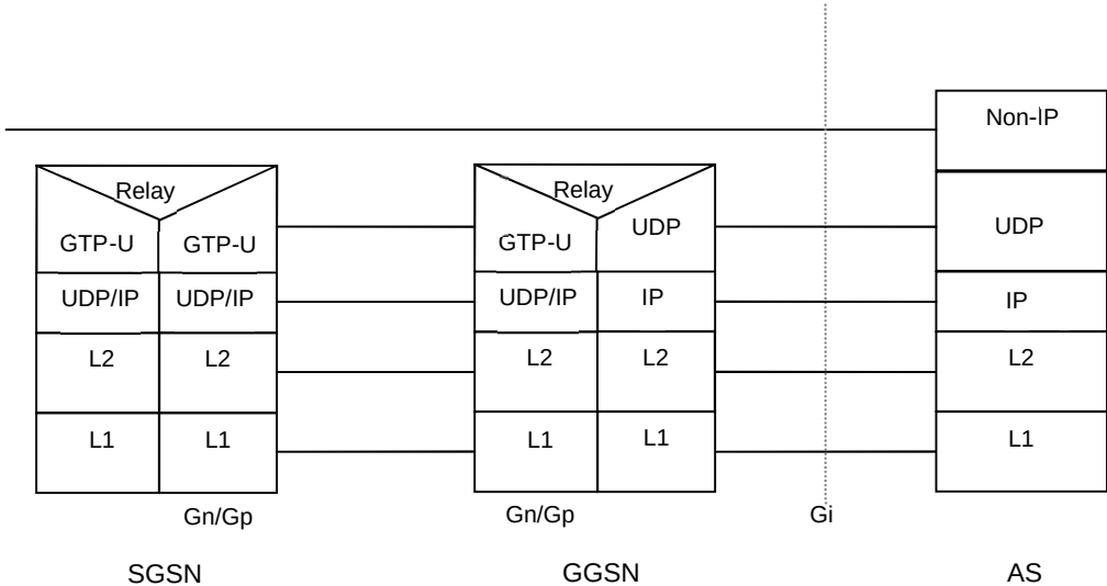
Figure 11.9: Protocol configuration for Non-IP data (user plane) using Gi PtP tunneling.
