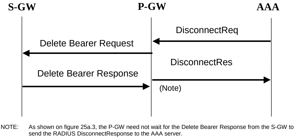
Figure 25a.3: AAA-initiated bearer termination with RADIUS
