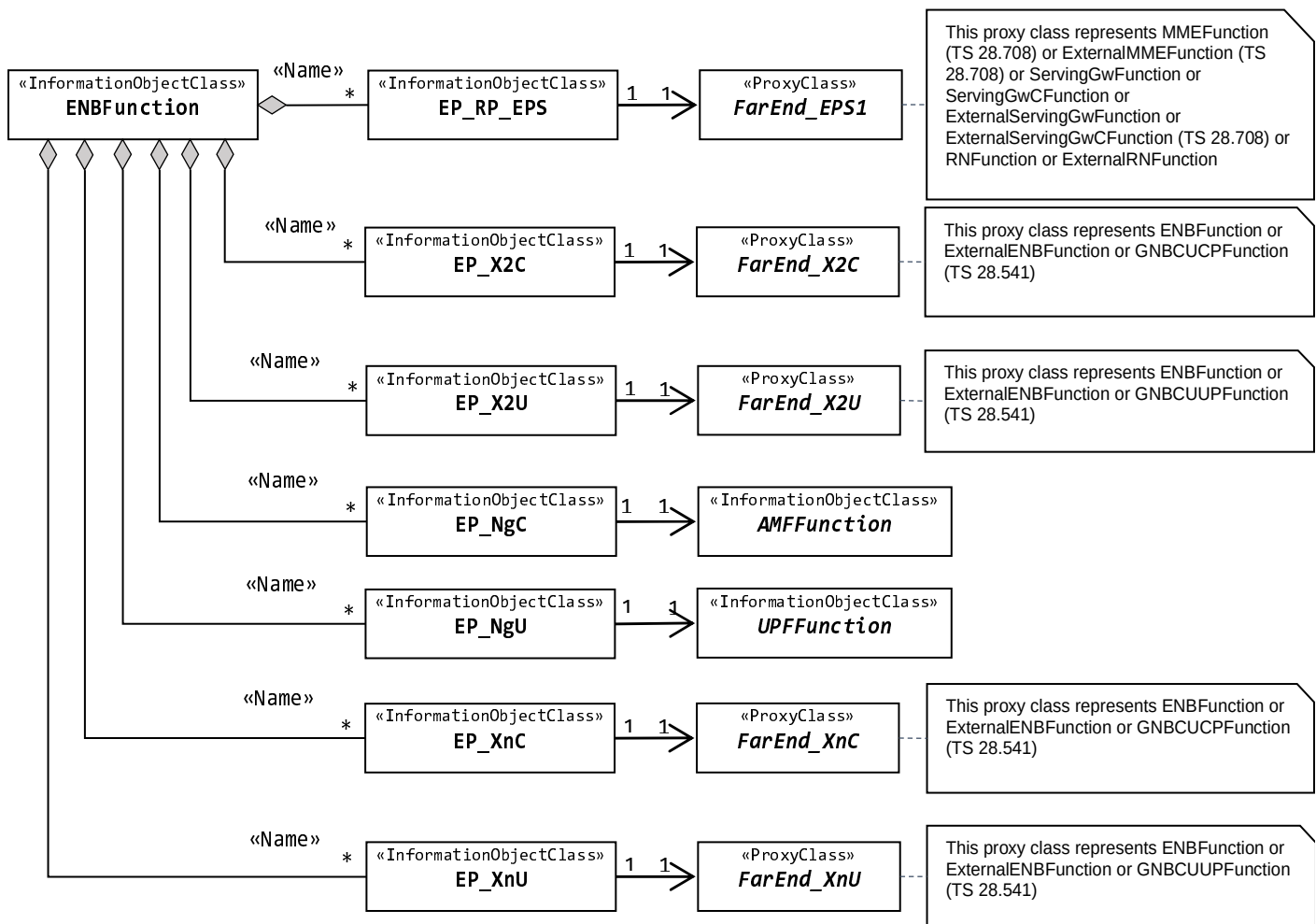
Figure 4.2.1-3: Transport view of E-UTRAN and ng-eNB NRM
