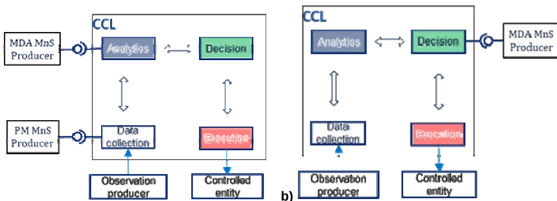
Figure 5.1.2.2-2: Management services used as implementations of CCL steps: a) MDA MnS and PM MnS job the respective implementations of the analysis and data collection steps; and b) MDA MnS as the implementation of the decision step
