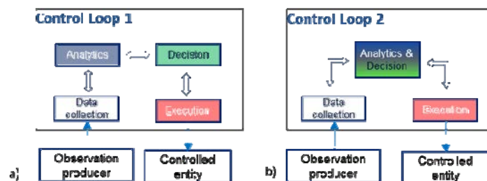
Figure 4.2-1: Steps of a Control Loop a) the four functional steps; and b) 2 steps combined into a single management function
