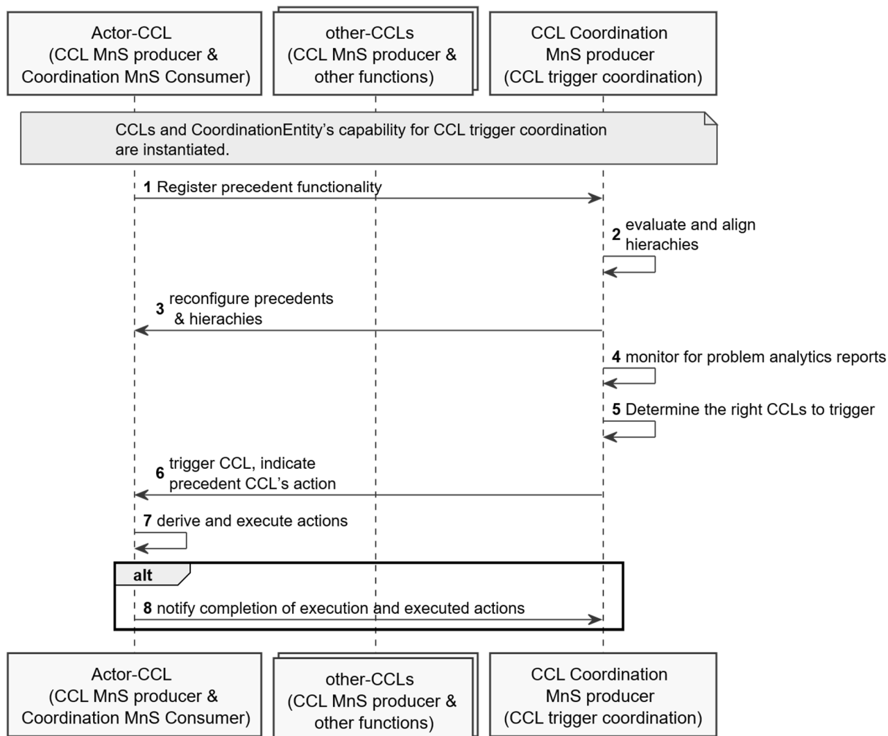
Figure 7.7-1: CCL-impact assessment and actual metric-value conflicts resolution
