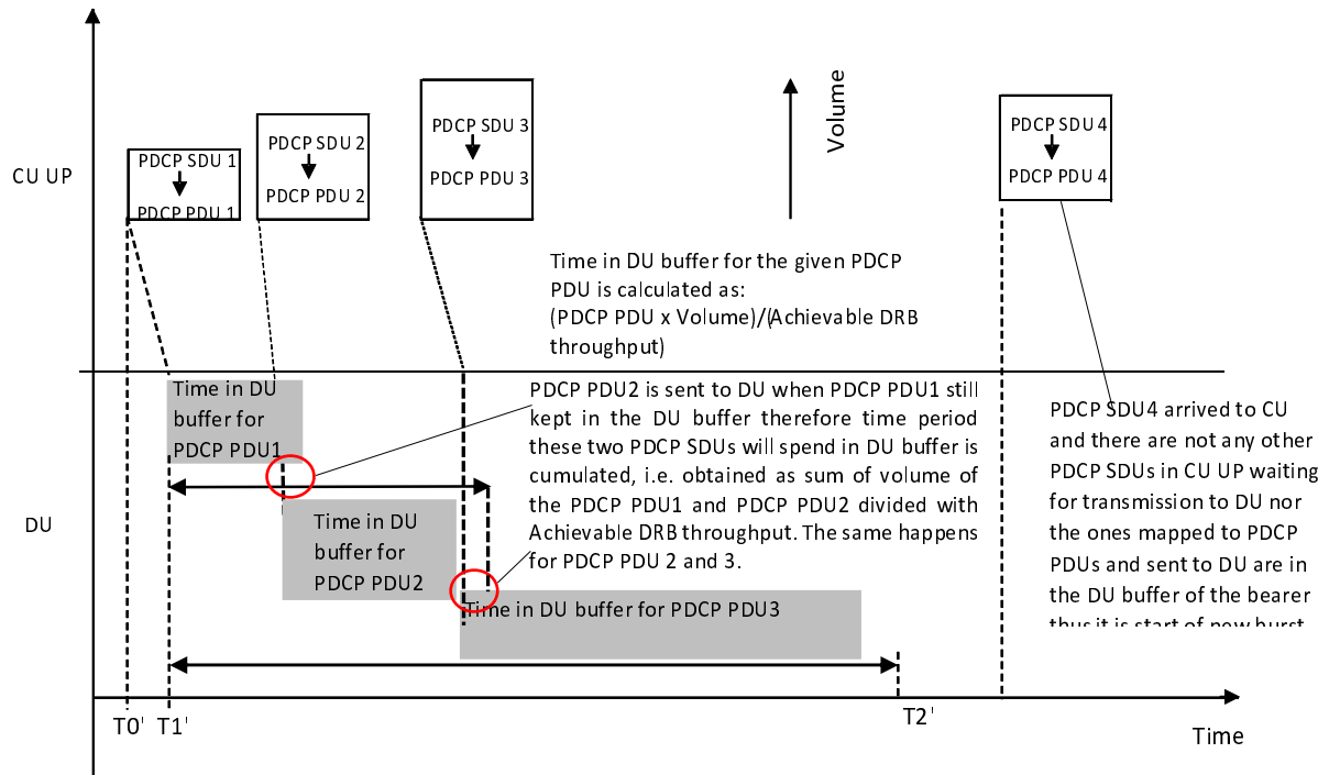
Figure 5.1.1.3.7-1 Average DL buffered UE throughput per DRB (SA, NSA option 3a)
