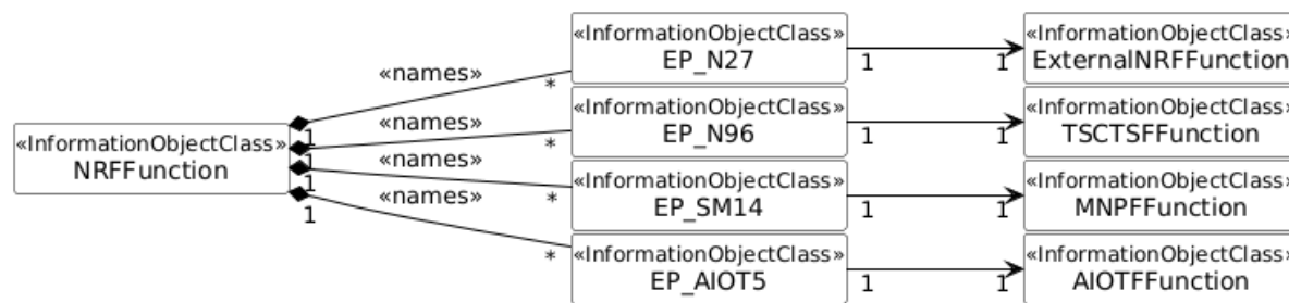
Figure 5.2.1.1-9: Transport view of NRF NRM
