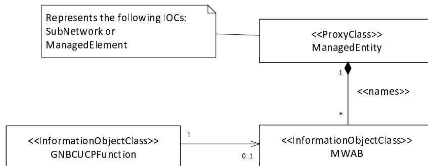
Figure 4.2.1.1-24: NRM fragment for MWAB
