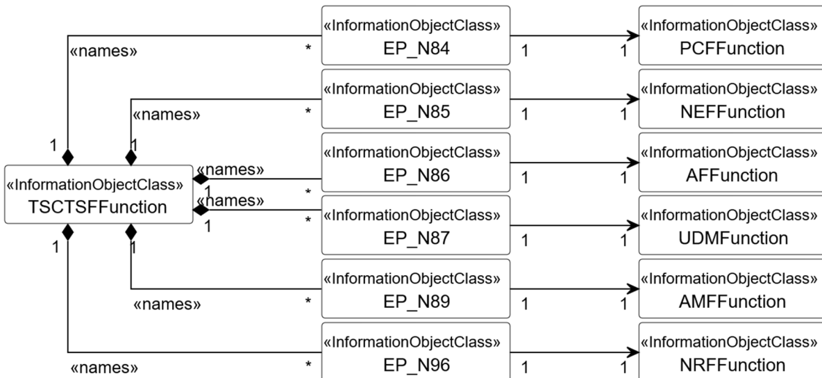
Figure 5.2.1.1-32: Transport view of TSCTSFFunction NRM fragment
