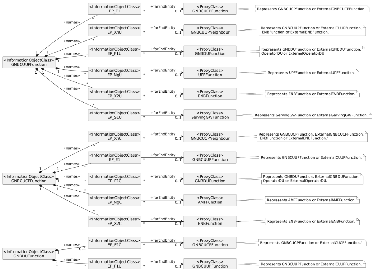
Figure 4.2.1.1-2: NRM for EPs for all deployment scenarios
