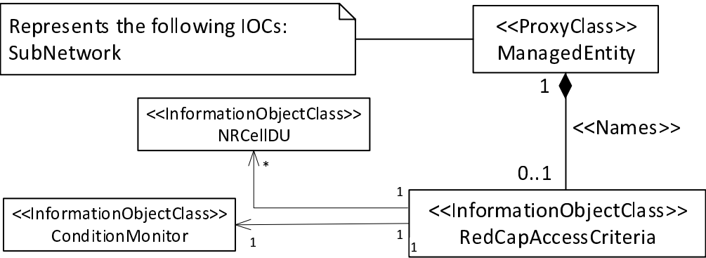
Figure 4.2.1.1-26: NRM fragment for RedCap Access
