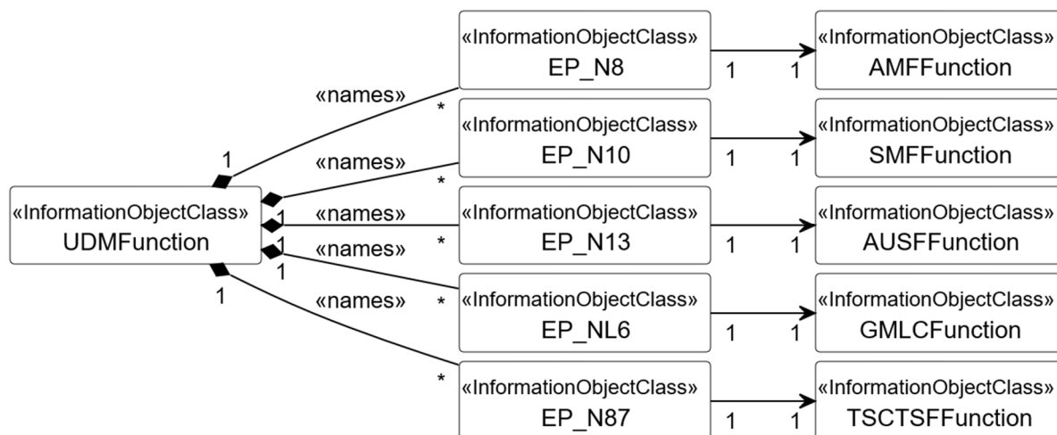
Figure 5.2.1.1-8: Transport view of UDM NRM
