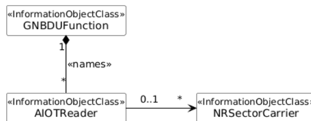
Figure 4.2.1.1-25: NRM relationship fragment for AIOT
