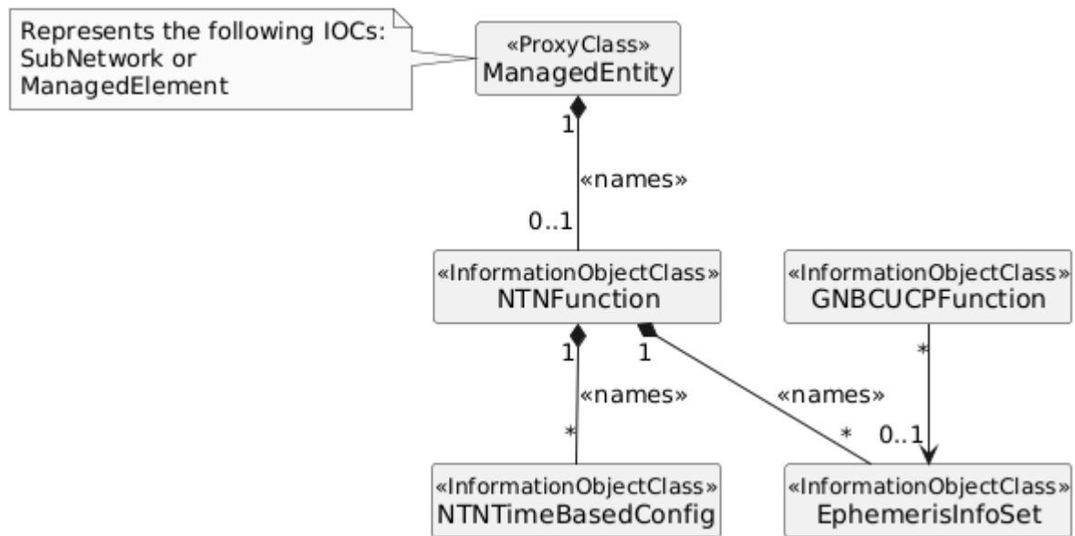
Figure 4.2.1.1-21: NRM fragment to support NTN management
