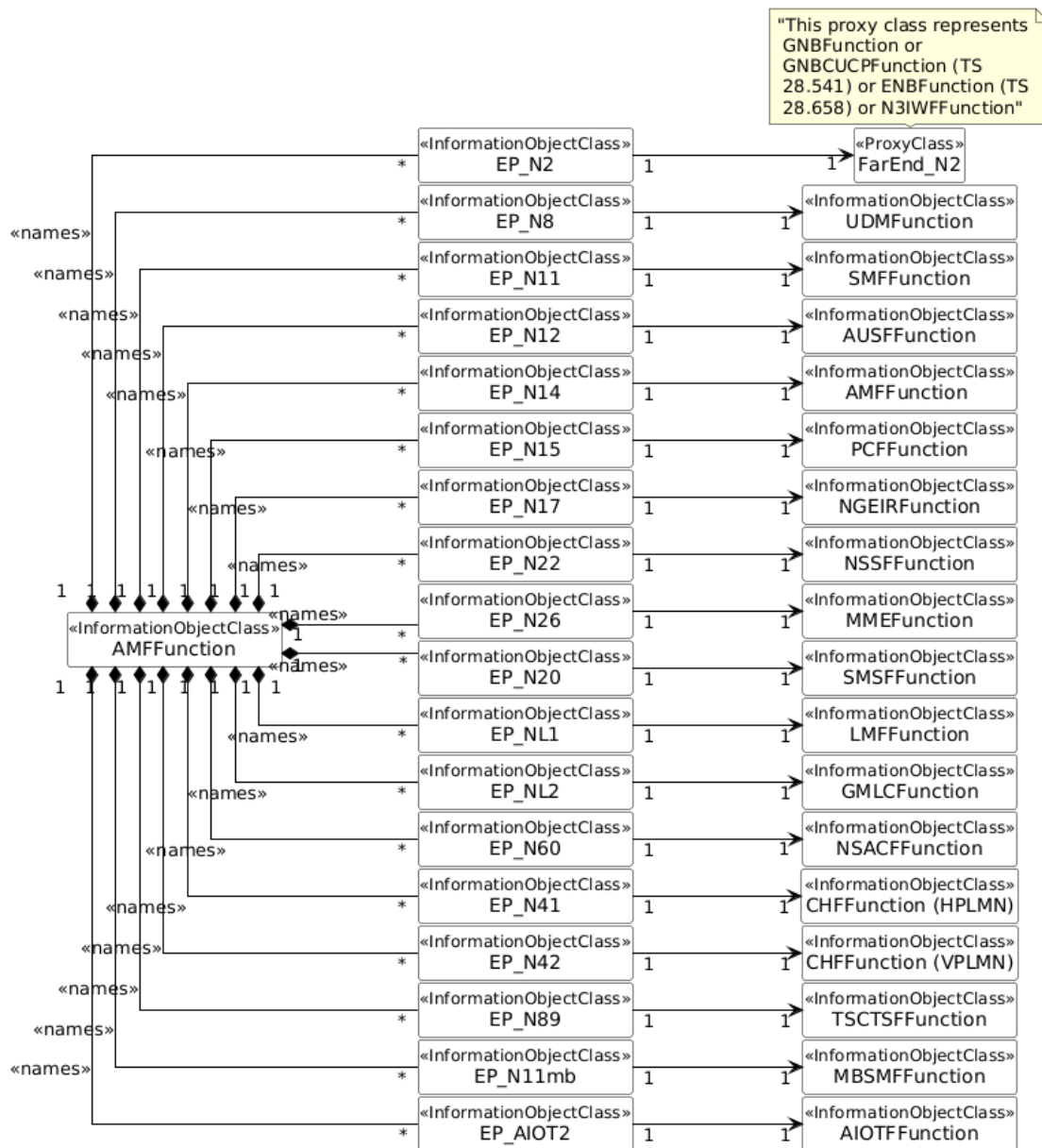
Figure 5.2.1.1-2: Transport view of AMF NRM
