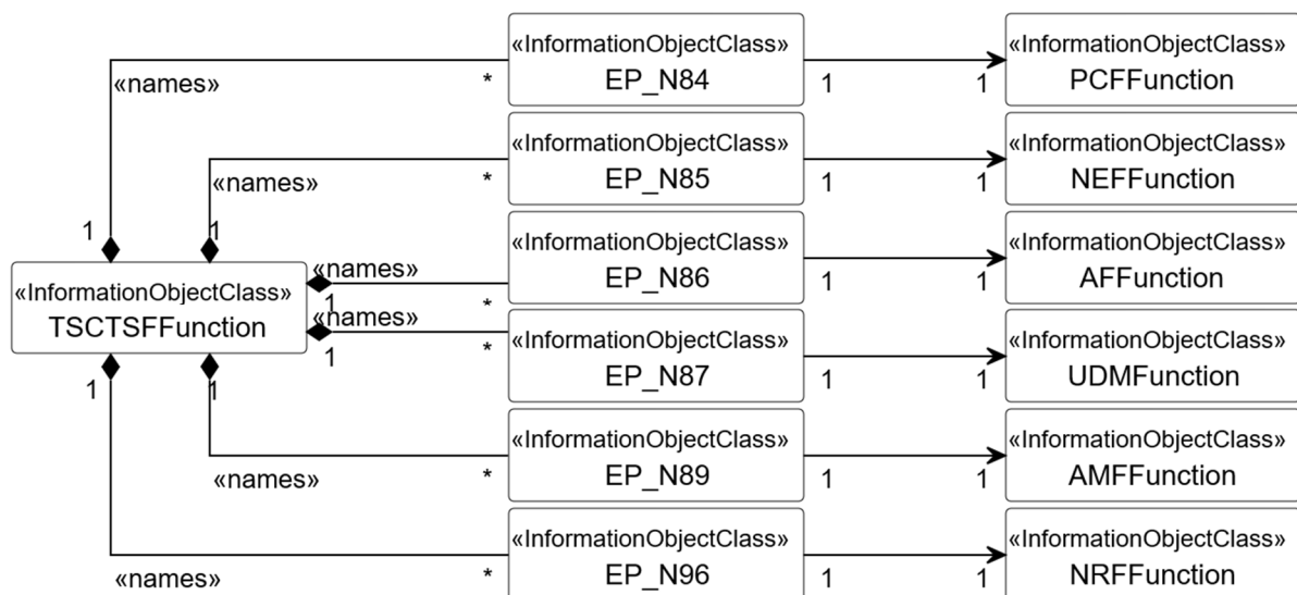
Figure 5.2.1.1-32: Transport view of TSCTSFFunction NRM fragment
