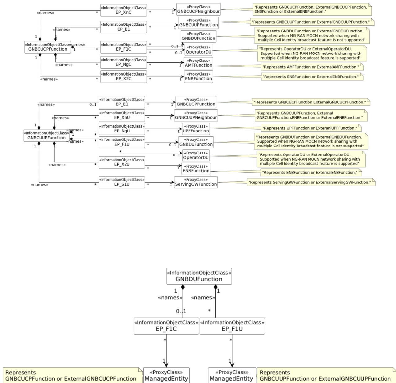
Figure 4.2.1.1-2: NRM for EPs for all deployment scenarios
