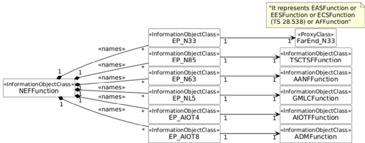
Figure 5.2.1.1-22: Transport view of NEF NRM
