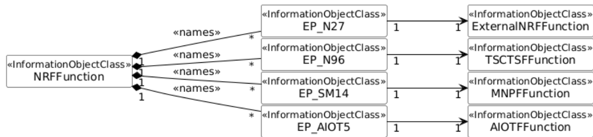
Figure 5.2.1.1-9: Transport view of NRF NRM
