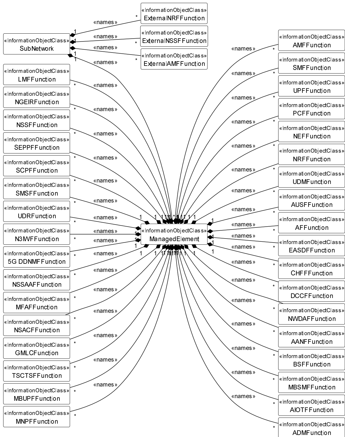
Figure 5.2.1.1-1: 5GC NRM containment/naming relationship
