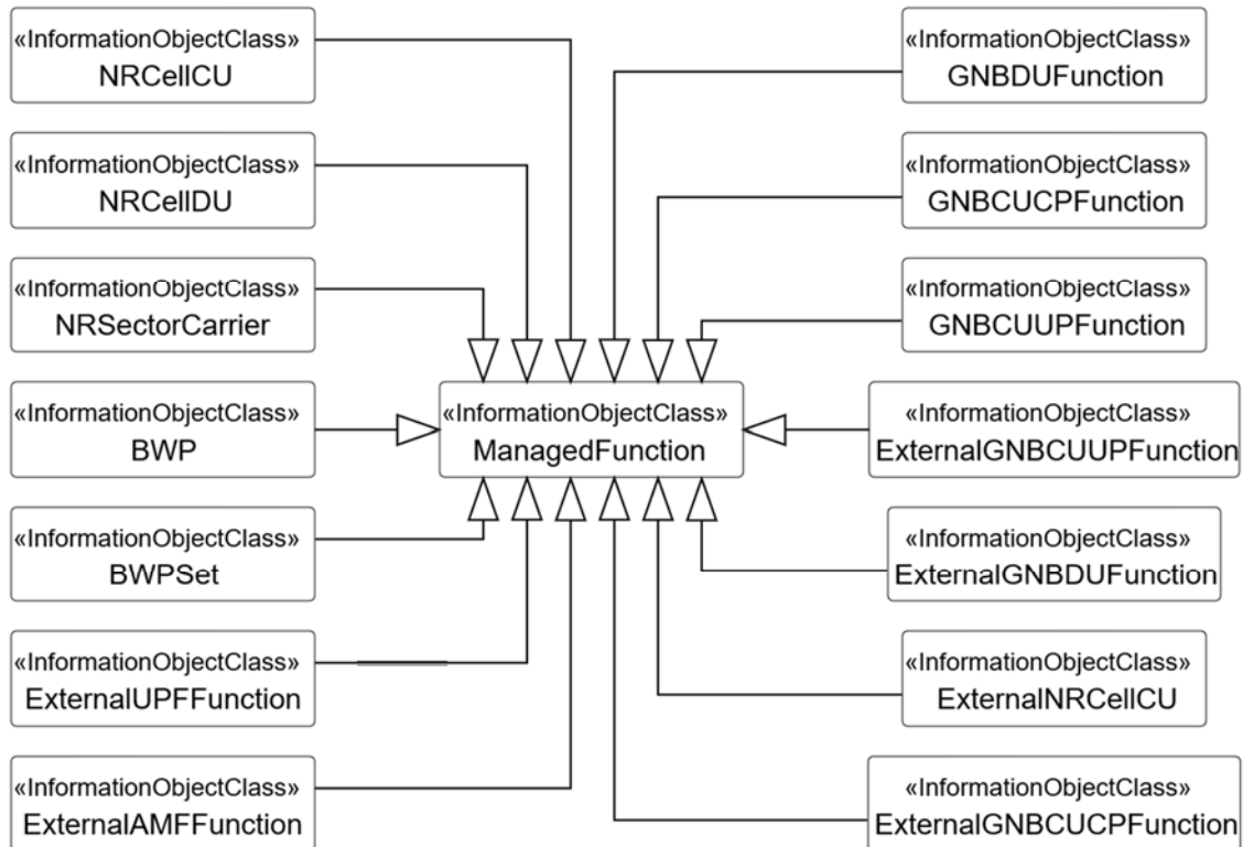
Figure 4.2.1.2-1: NR NRM fragment in all deployment scenarios
