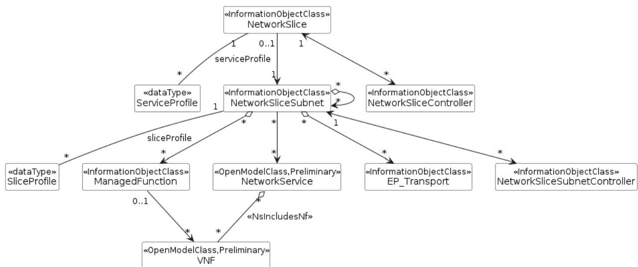
Figure 6.2.1-1: Network slice NRM fragment relationship
