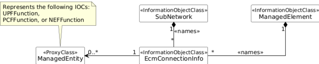
Figure 5.2.1.1-25: EcmConnectionInfo NRM
