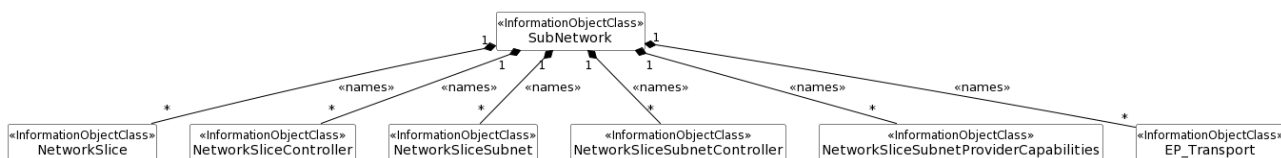
Figure 6.2.1-3: Containment relationship for network slice fragment
