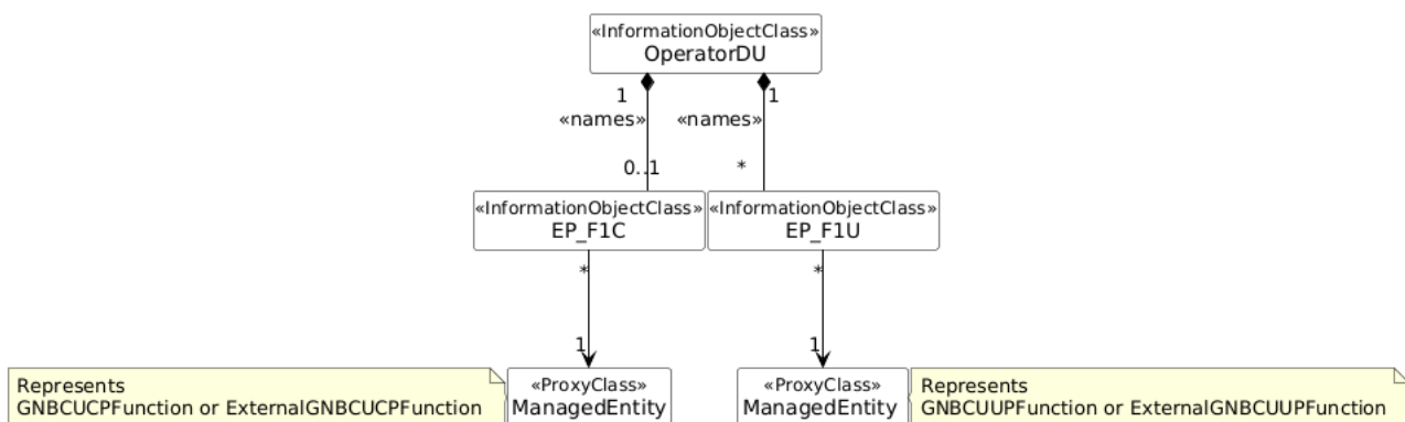
Figure 4.2.1.1-18: NRM fragment for F1 related EPs to support individual F1 interface for NG-RAN MOCN network sharing with multiple cell identity broadcast feature
