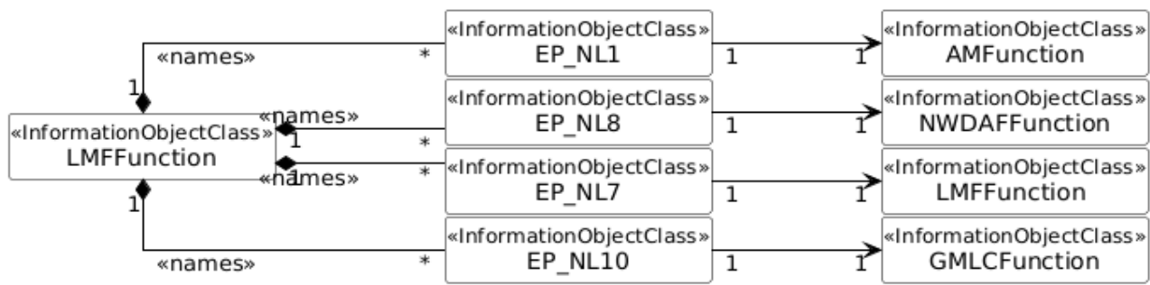
Figure 5.2.1.1-12: Transport view of LMF NRM
