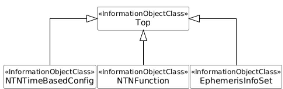
Figure 4.2.1.2-11: NRM fragment for NTN management
