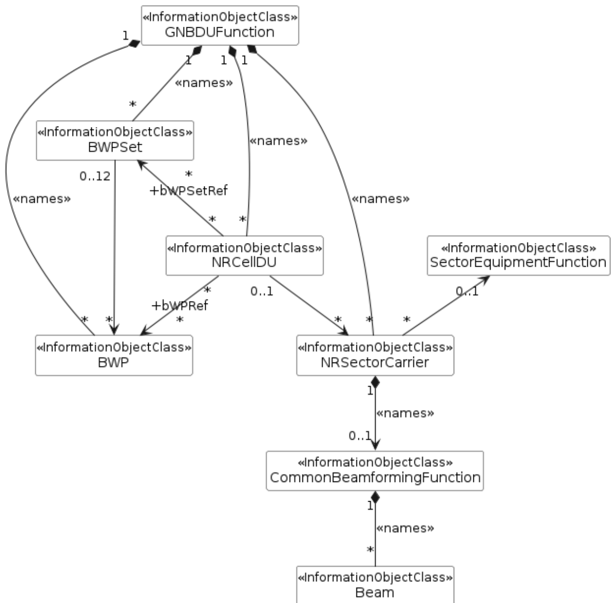
Figure 4.2.1.1-3: NRM for <<IOC>>NRSectorCarrier, <<IOC>>BWP, <<IOC>>SectorEquipmentFunction and <<IOC>> BWPSet for all deployment scenarios
