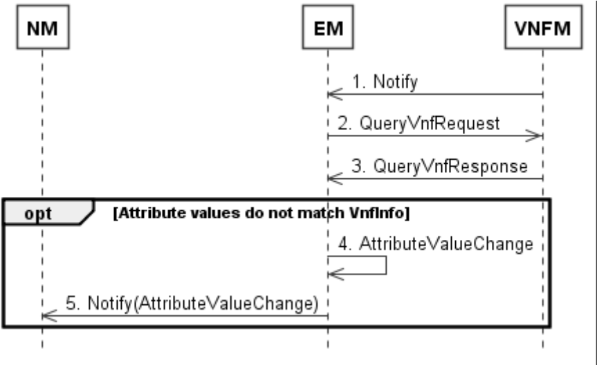
Figure 4.7-1: VNF instance information synchronization
