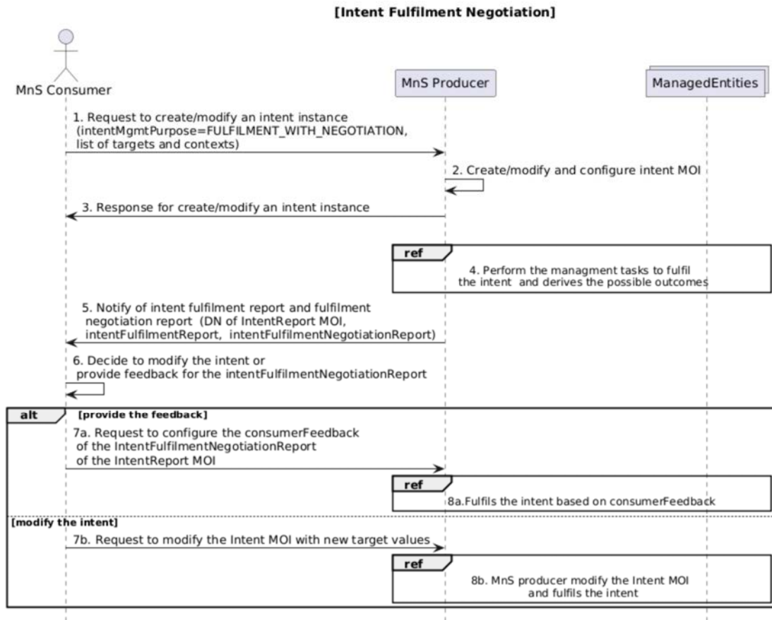
Figure 6.3.9-1: Procedure for intent negotiation during fulfilment phase
