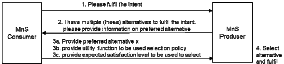
Figure 5.3.9.5-1: MnS consumer advises the MnS producer on the preferences among alternatives at the MnS producer
