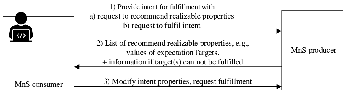
Figure 5.3.9.4-1: Enabling the MnS consumer to request and receive a recommendation on the possible fulfillable intent properties prior to or in case of failure of fulfilment
