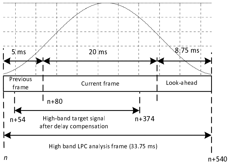
Figure 47: SWB Highband target signal buffers
