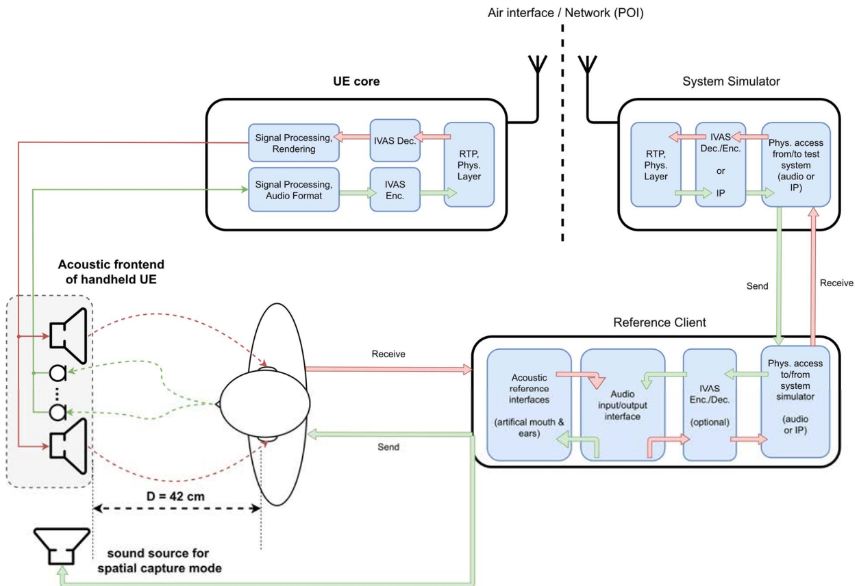
Figure 10: Handheld hands-free UE and test equipment
