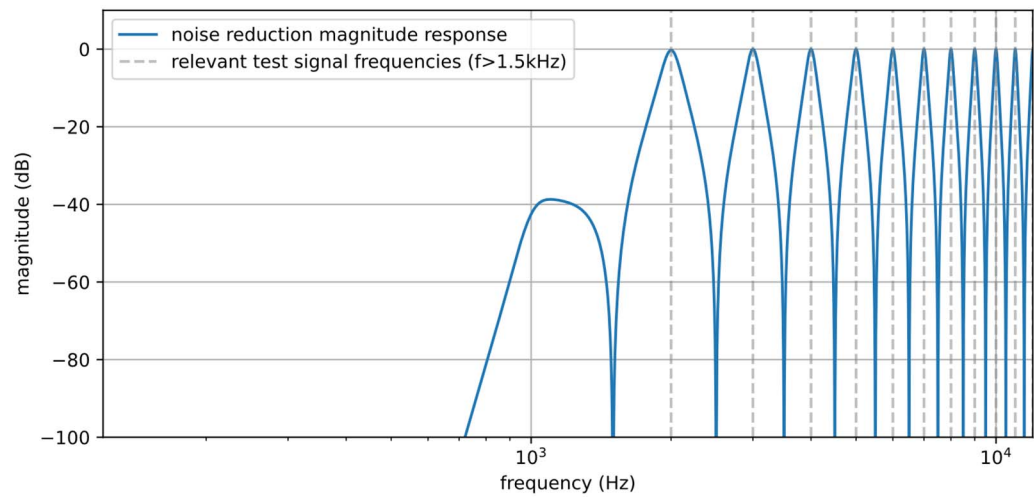
Figure D-1: Frequency response of noise reduction filter
