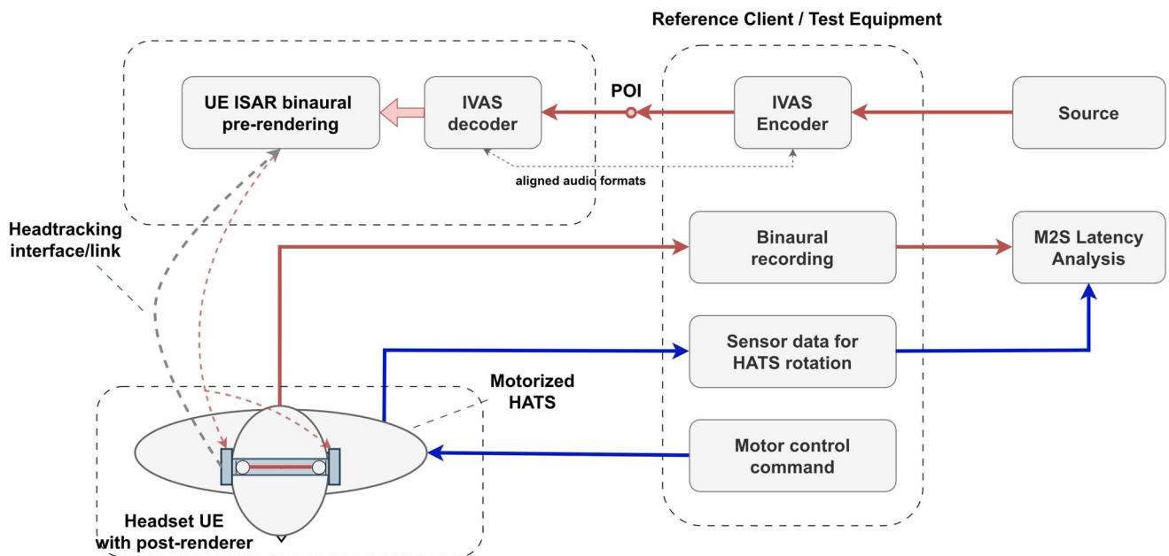
Figure 18b: Setup for measuring M2S latency with IVAS split rendering (ISAR) using a motorized HATS
