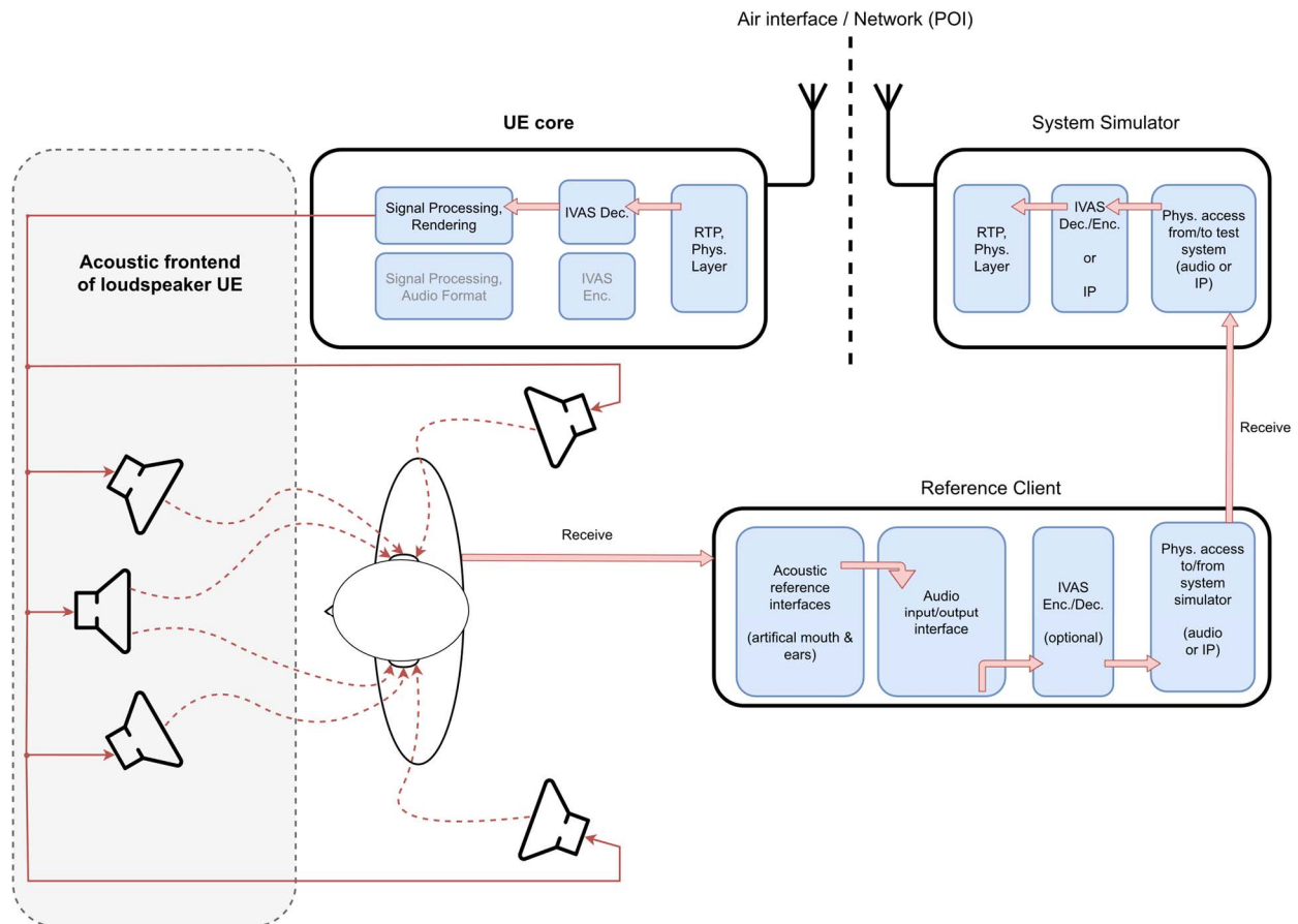
Figure 14: Loudspeaker hands-free UE and test equipment
