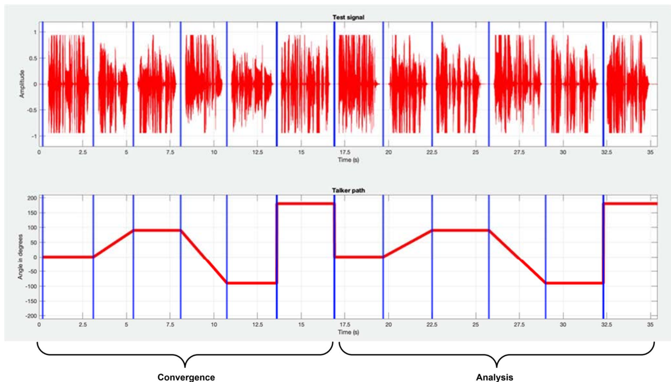
Figure 17a: Sentence directions in the test signal
