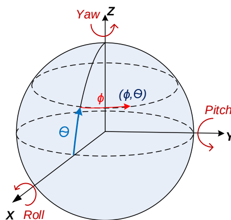
Figure 0: Spherical coordinate system
