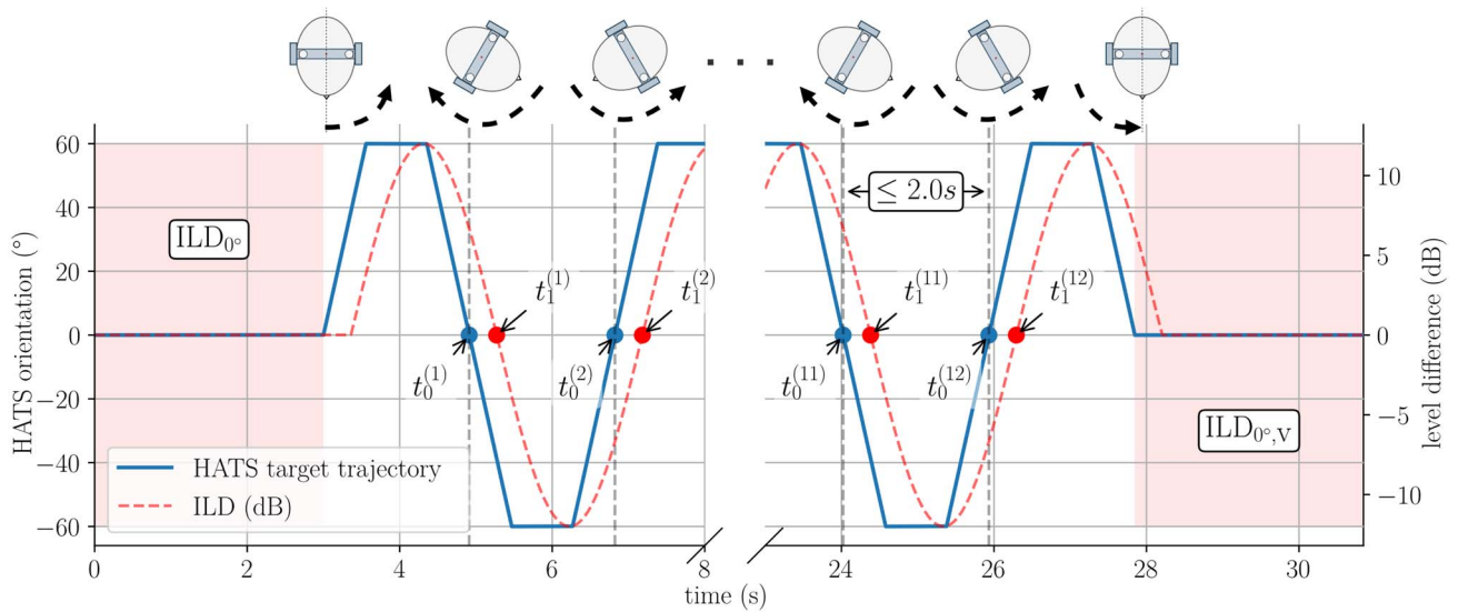
Figure 18d: Example setup for measuring M2S latency using a motorized HATS
