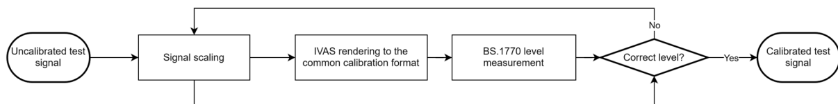
Figure 16: Test signal input level adjustment procedure for receiving tests
