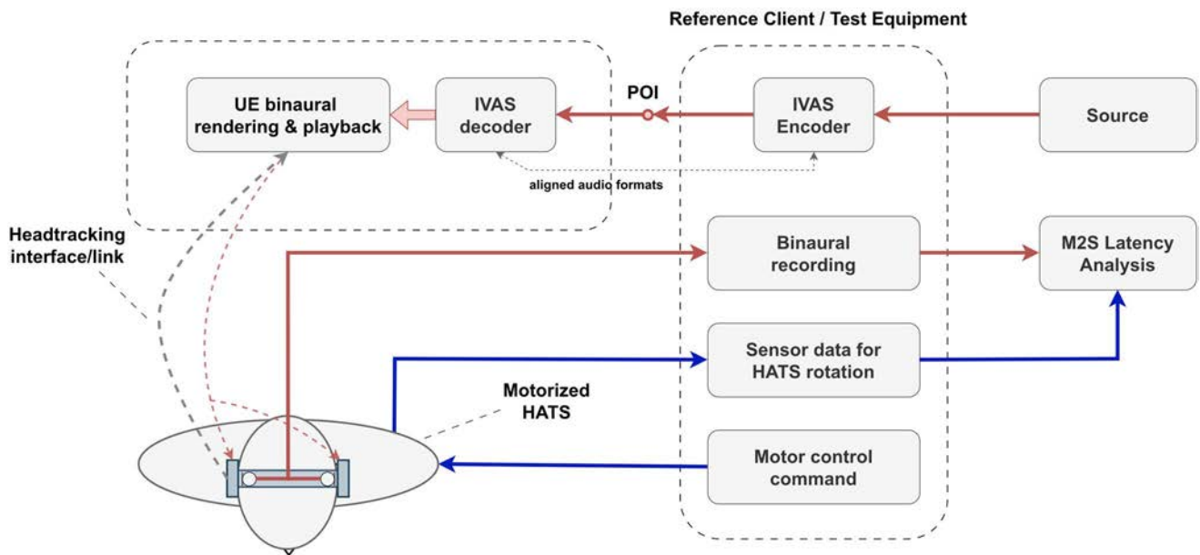
Figure 18a: Setup for measuring M2S latency using a motorized HATS
