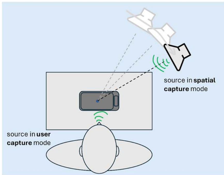
Figure 13: Sound source positioning for Table-mounted UE tests
