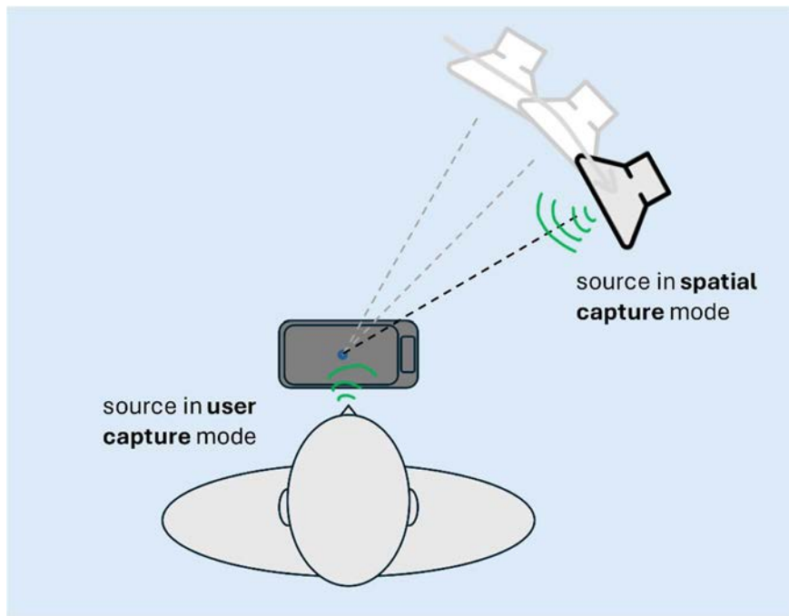
Figure 11: Sound source positioning for Handheld UE tests
