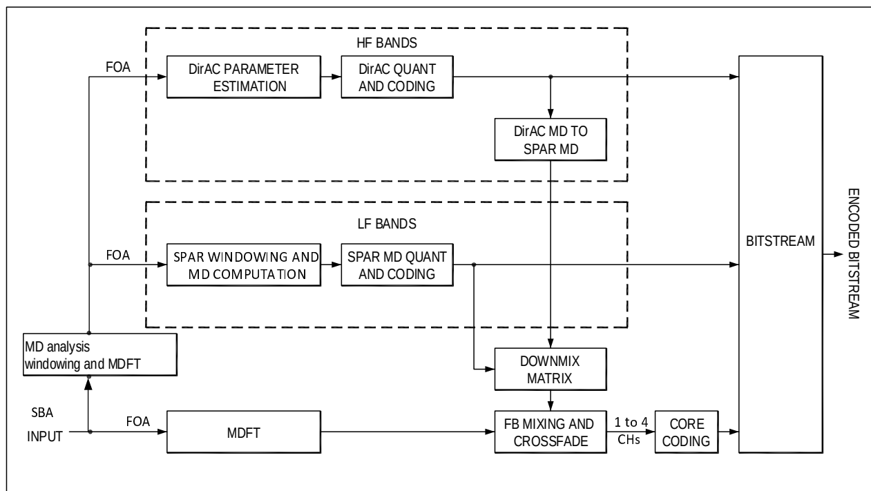
Figure 5.4-2: FOA signal coding at all bitrates and HOA2, HOA3 signal coding at 256 kbps
