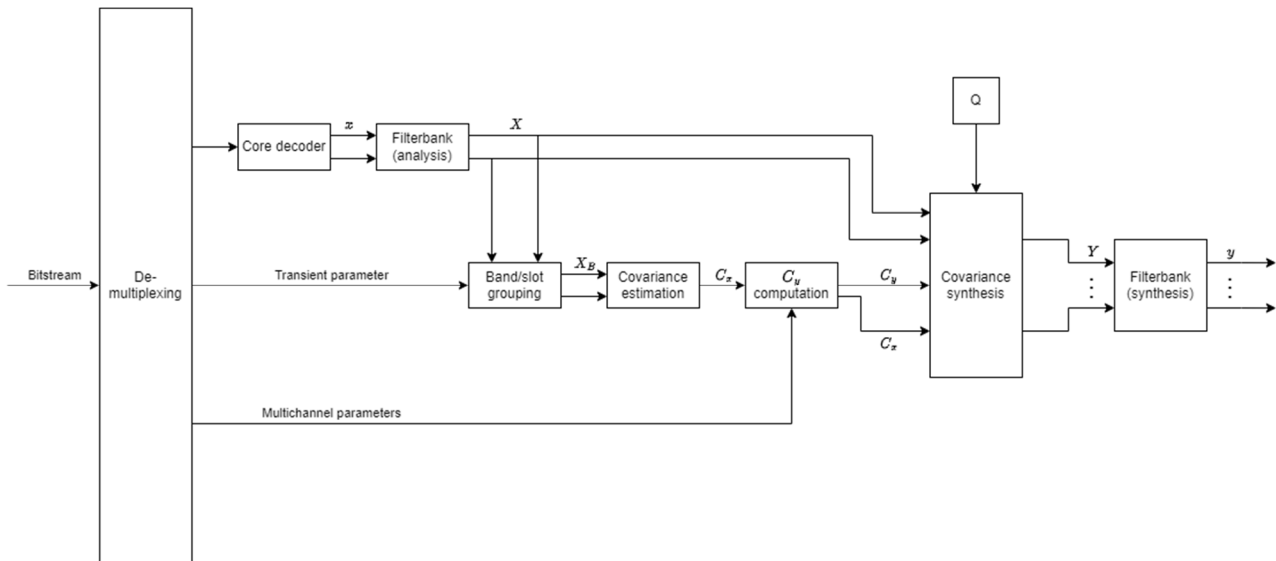
Figure 6.7-1: ParamMC Decoder
