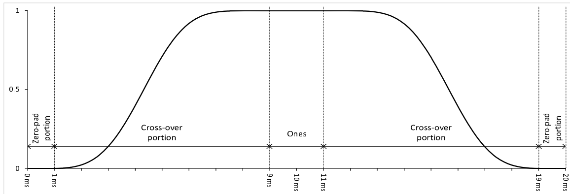
Figure 5.7-1: KBD window used in MDCT based LFE channel codec
