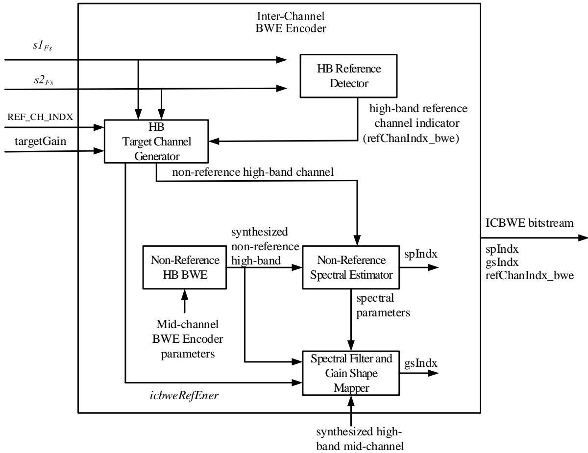
Figure 5.3-4: Block diagram of the IC-BWE Encoder
