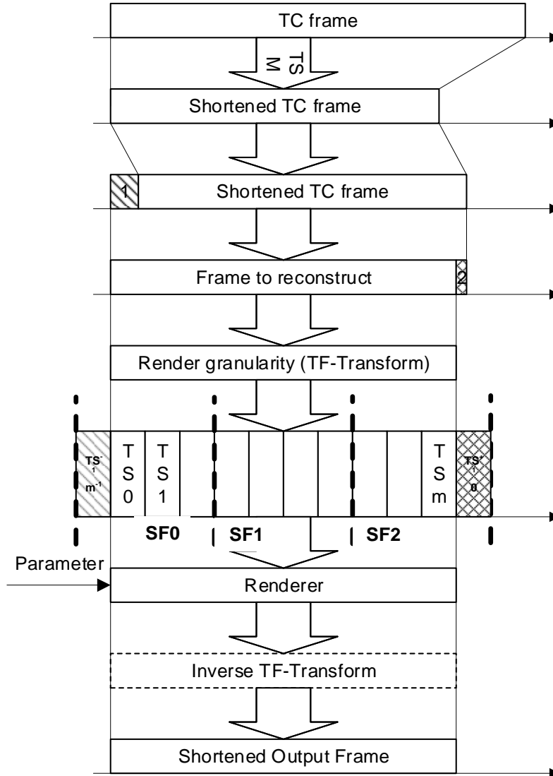
Figure 6.2-21: TSM local subframe adaption
