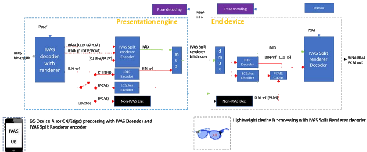
Figure 4.5-2: IVAS Split Rendering functions
