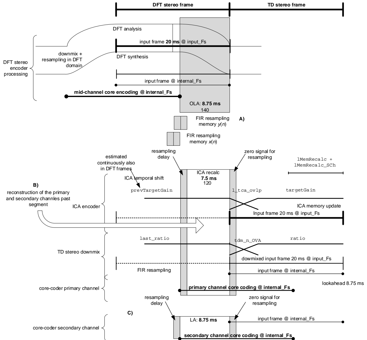
Figure 5.3-43: Flow chart illustrating operations upon switching from DFT stereo to TD stereo
