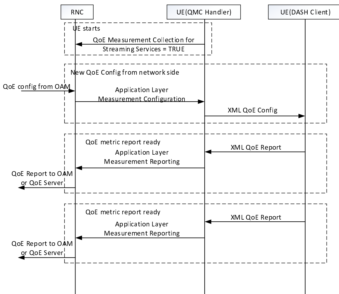
Figure L-1: Example signalling diagram for UMTS
