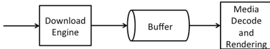
Figure 11-1 Simple client model
