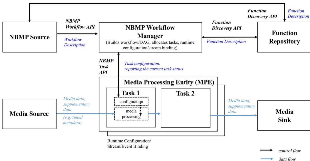
Figure X.1 – NBMP reference architecture
