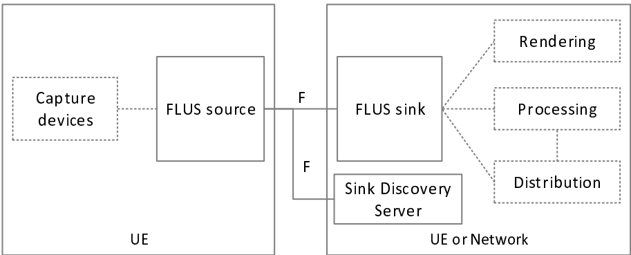
Figure 4.2-1: FLUS architecture
