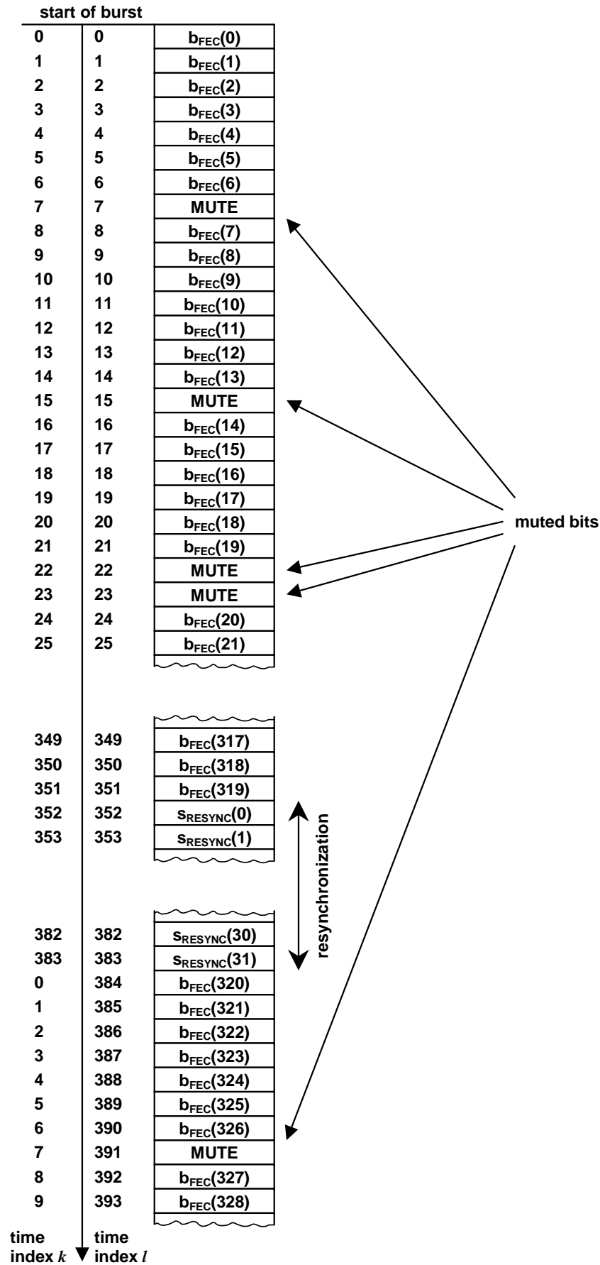
Figure 5 – Organization of the bit-stream b_{\text{OUT}} to the interleaver
